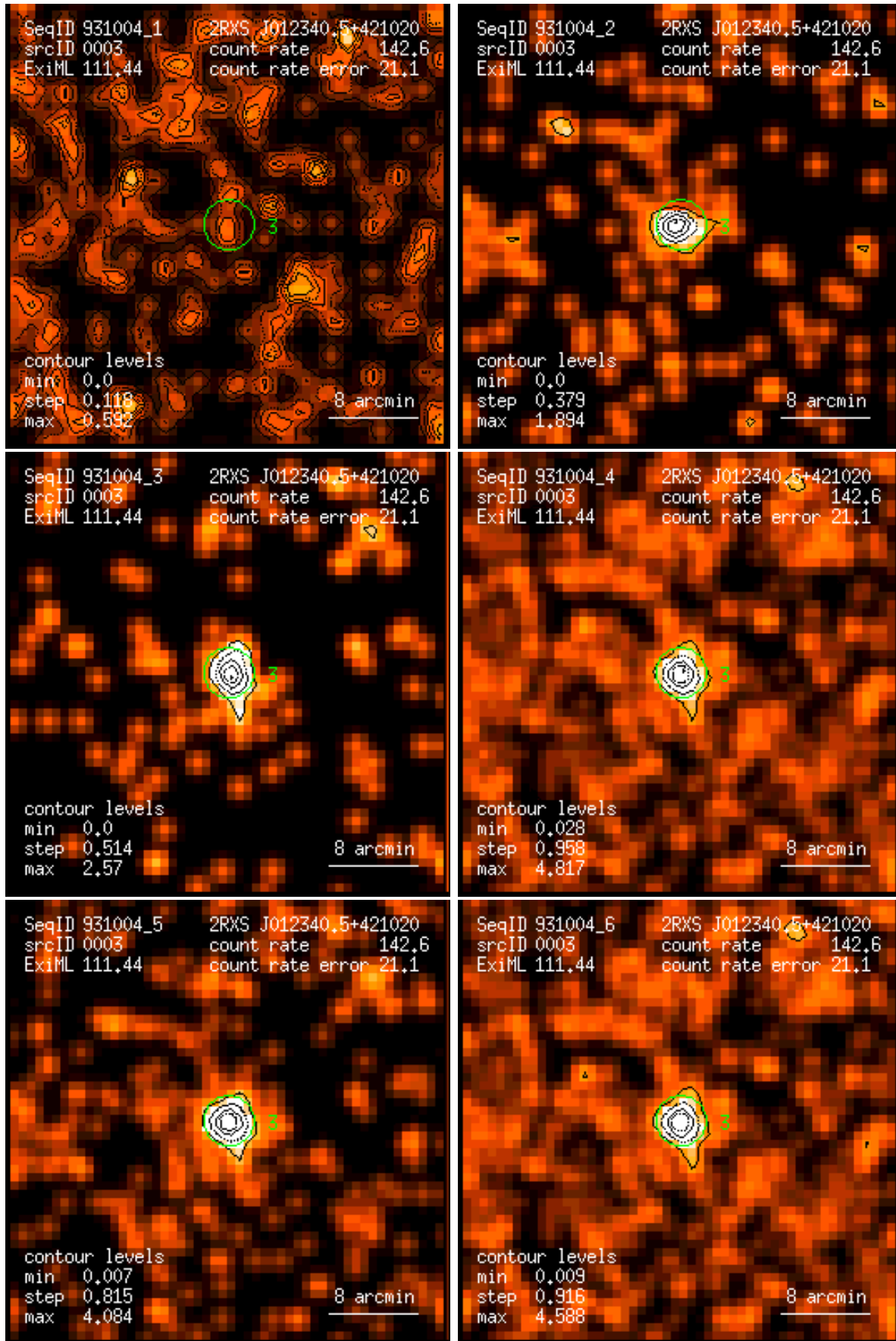
Figure 3: RASS 931004: detection 0003: band rate images, Gaussian filter: (1) PSPC channels 11 – 41, (2) 52 – 90, (3) 91 – 201, (4) 11 – 235, (5) 52 – 201, (6) 11 – 201. Broad band rates in counts/ks. Band rate contour levels in counts/ks/arcmin 2 .
