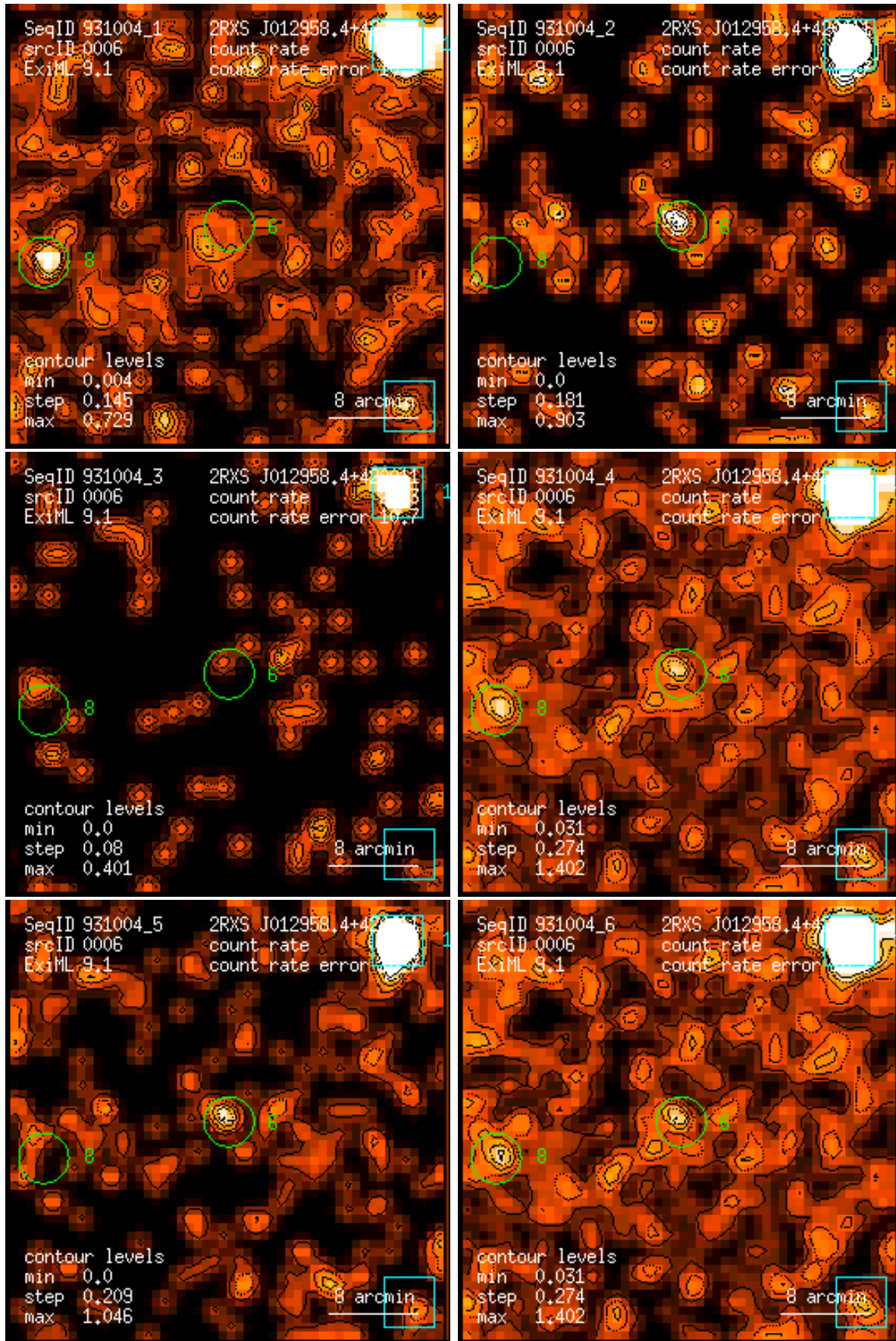
Figure 6: RASS 931004: detection 0006: band rate images, Gaussian filter: (1) PSPC channels 11 – 41, (2) 52 – 90, (3) 91 – 201, (4) 11 – 235, (5) 52 – 201, (6) 11 – 201. Broad band rates in counts/ks. Band rate contour levels in counts/ks/arcmin 2 .
