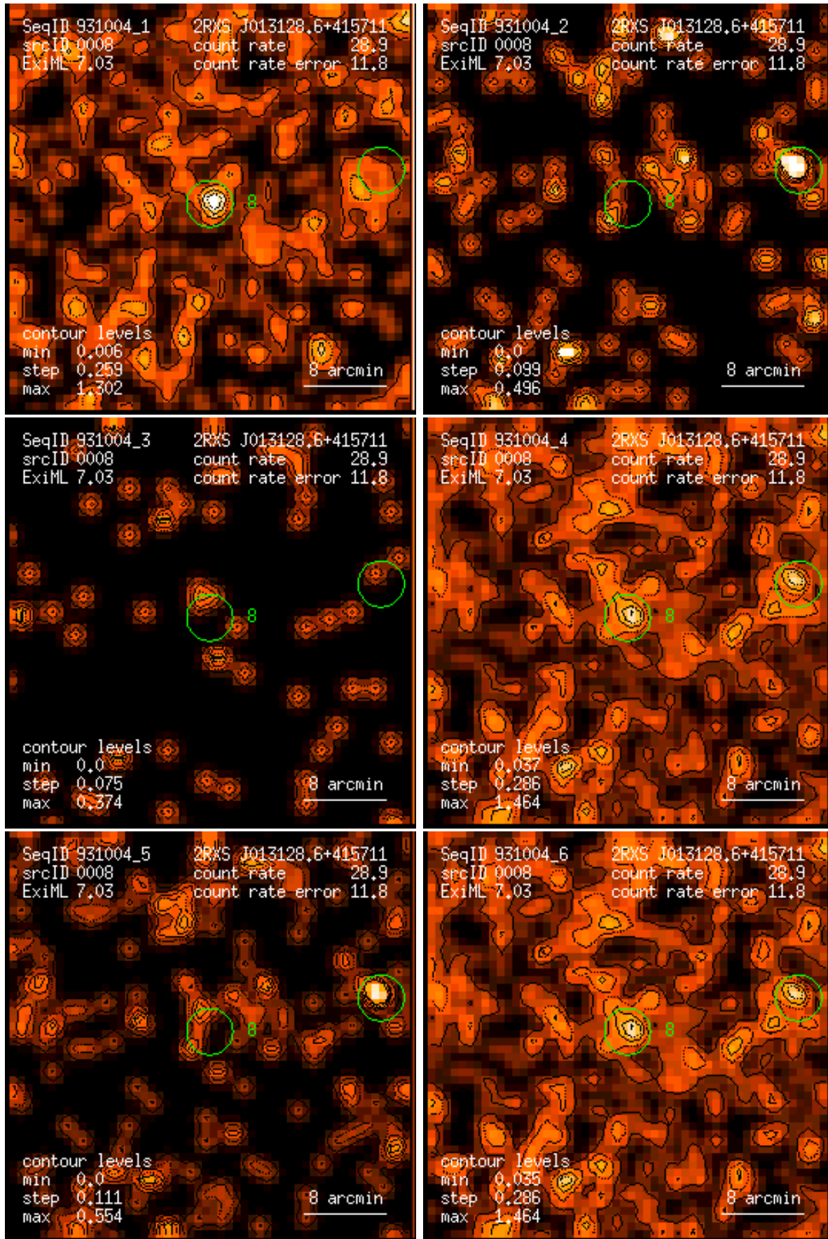
Figure 8: RASS 931004: detection 0008: band rate images, Gaussian filter: (1) PSPC channels 11 – 41, (2) 52 – 90, (3) 91 – 201, (4) 11 – 235, (5) 52 – 201, (6) 11 – 201. Broad band rates in counts/ks. Band rate contour levels in counts/ks/arcmin 2 .
