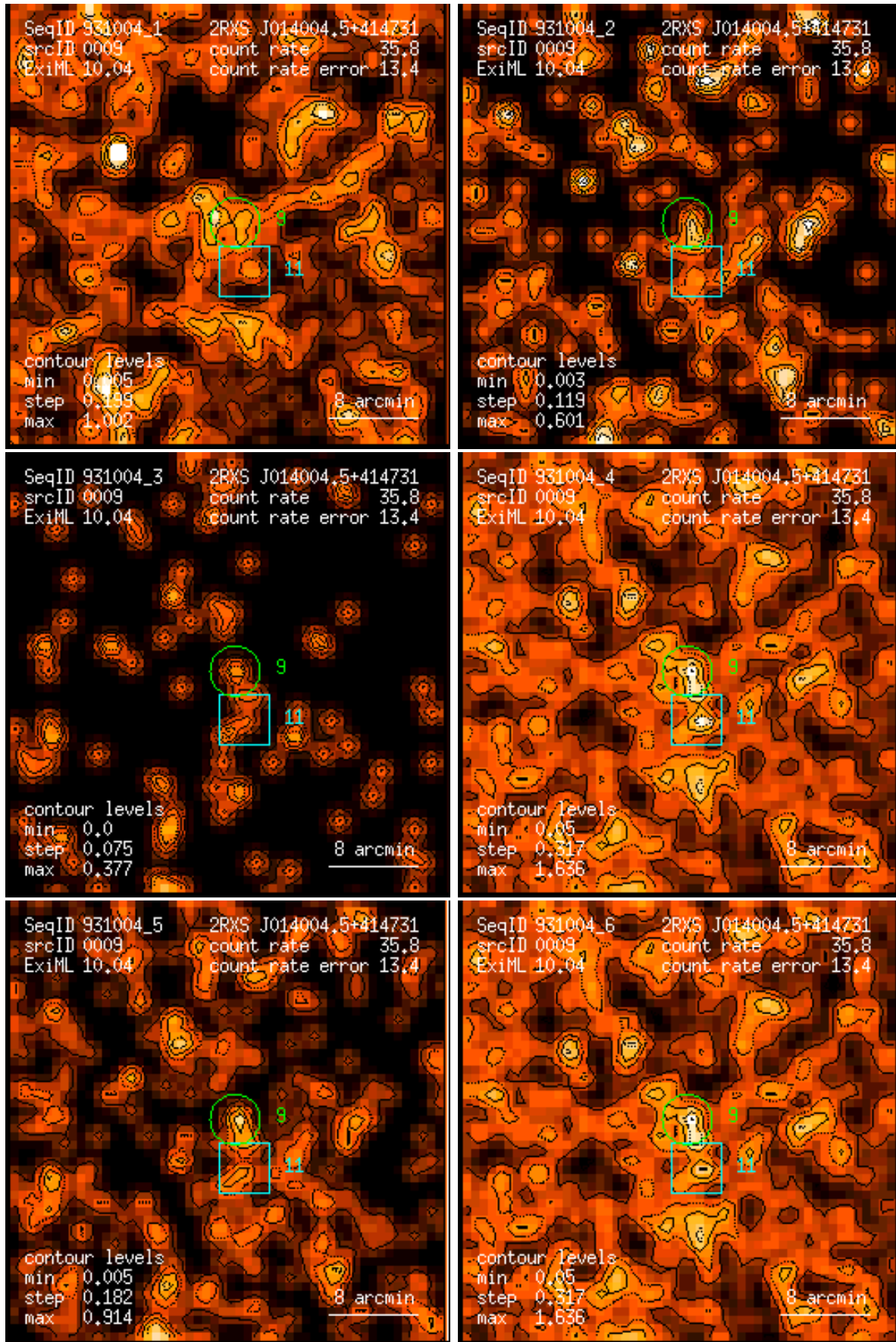
Figure 9: RASS 931004: detection 0009: band rate images, Gaussian filter: (1) PSPC channels 11 – 41, (2) 52 – 90, (3) 91 – 201, (4) 11 – 235, (5) 52 – 201, (6) 11 – 201. Broad band rates in counts/ks. Band rate contour levels in counts/ks/arcmin 2 .
