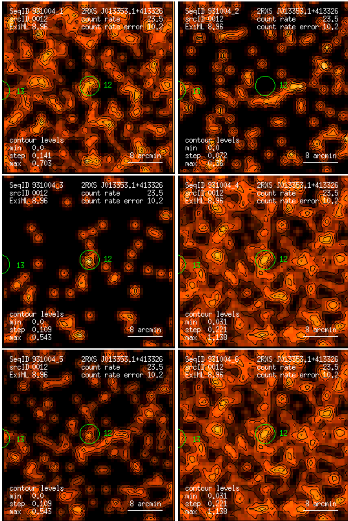
Figure 12: RASS 931004: detection 0012: band rate images, Gaussian filter: (1) PSPC channels 11 – 41, (2) 52 – 90, (3) 91 – 201, (4) 11 – 235, (5) 52 – 201, (6) 11 – 201. Broad band rates in counts/ks. Band rate contour levels in counts/ks/arcmin 2 .
