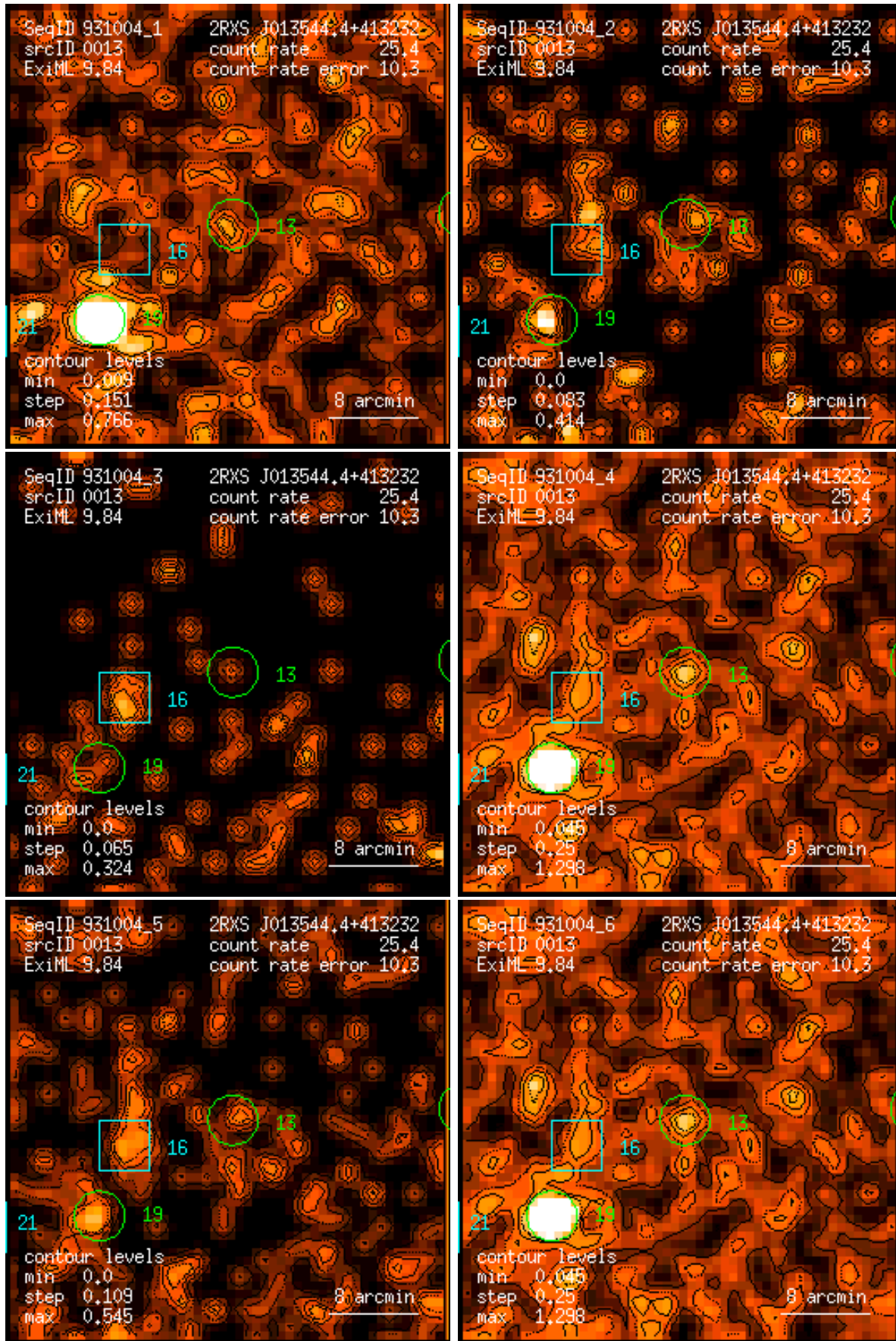
Figure 13: RASS 931004: detection 0013: band rate images, Gaussian filter: (1) PSPC channels 11 – 41, (2) 52 – 90, (3) 91 – 201, (4) 11 – 235, (5) 52 – 201, (6) 11 – 201. Broad band rates in counts/ks. Band rate contour levels in counts/ks/arcmin 2 .
