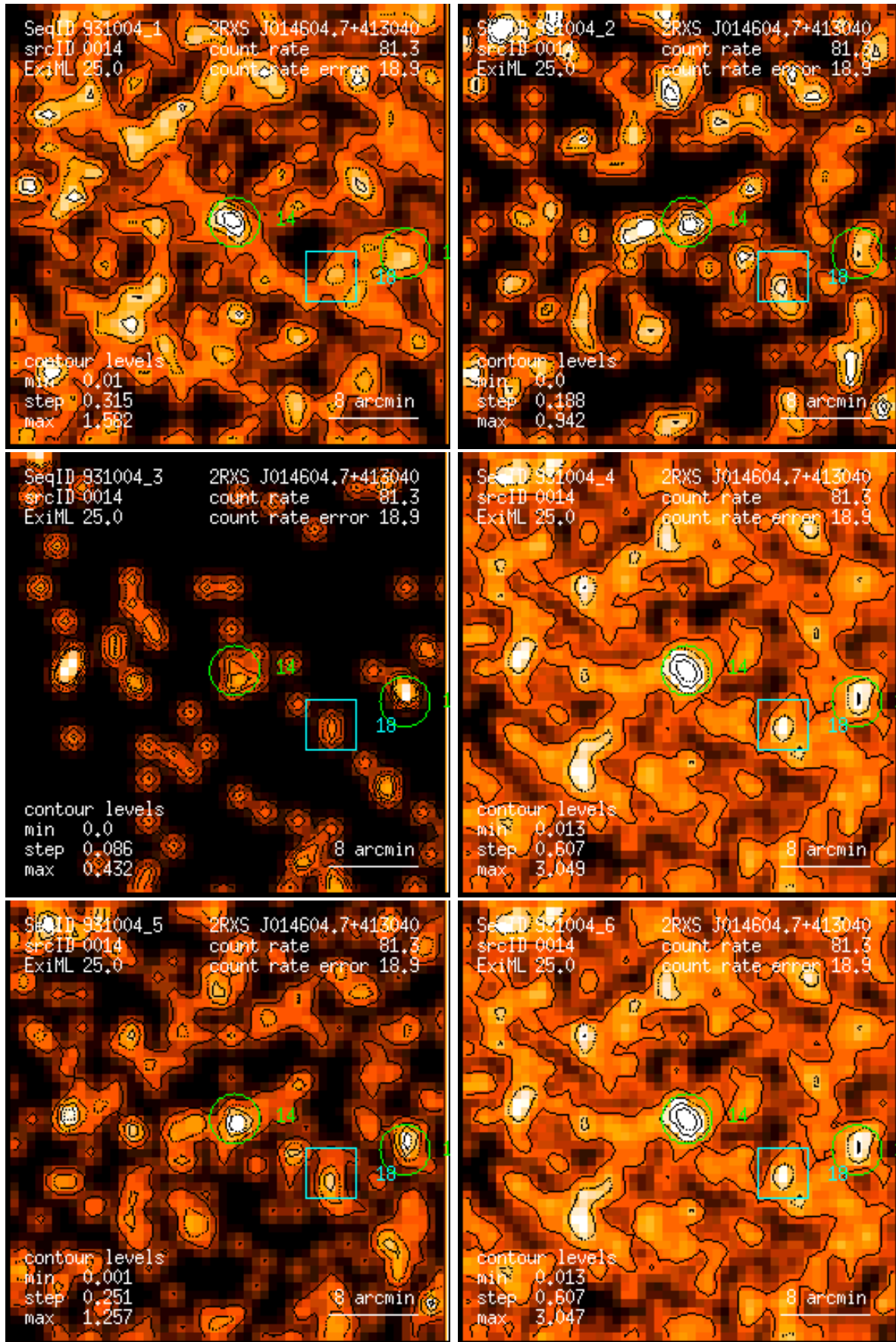
Figure 14: RASS 931004: detection 0014: band rate images, Gaussian filter: (1) PSPC channels 11 – 41, (2) 52 – 90, (3) 91 – 201, (4) 11 – 235, (5) 52 – 201, (6) 11 – 201. Broad band rates in counts/ks. Band rate contour levels in counts/ks/arcmin 2 .
