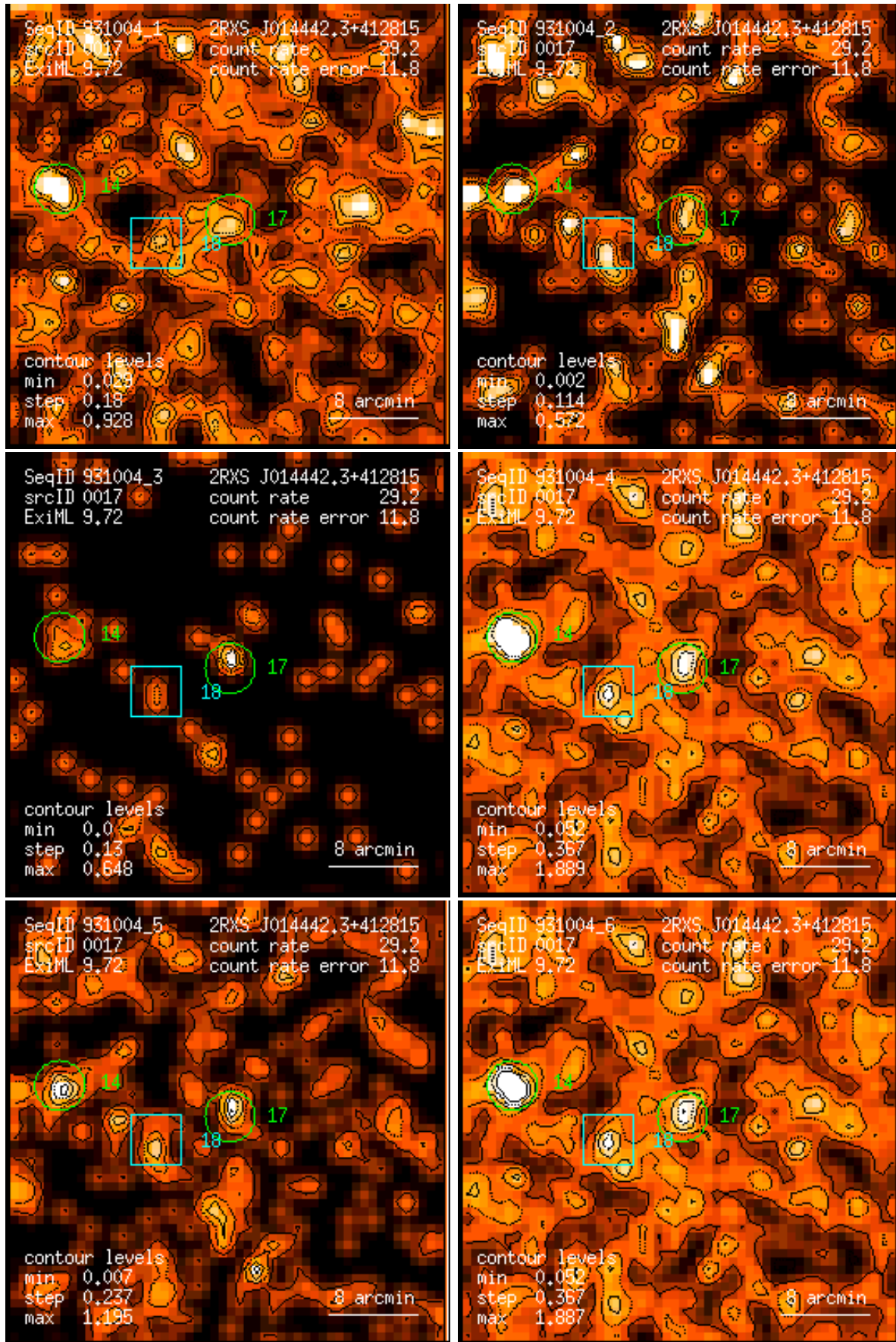
Figure 17: RASS 931004: detection 0017: band rate images, Gaussian filter: (1) PSPC channels 11 – 41, (2) 52 – 90, (3) 91 – 201, (4) 11 – 235, (5) 52 – 201, (6) 11 – 201. Broad band rates in counts/ks. Band rate contour levels in counts/ks/arcmin 2 .
