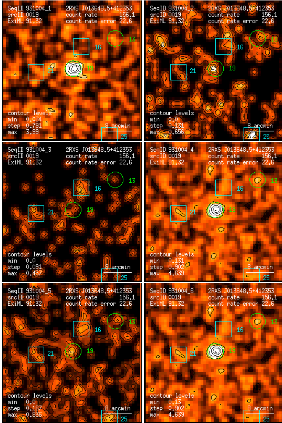
Figure 19: RASS 931004: detection 0019: band rate images, Gaussian filter: (1) PSPC channels 11 – 41, (2) 52 – 90, (3) 91 – 201, (4) 11 – 235, (5) 52 – 201, (6) 11 – 201. Broad band rates in counts/ks. Band rate contour levels in counts/ks/arcmin 2 .
