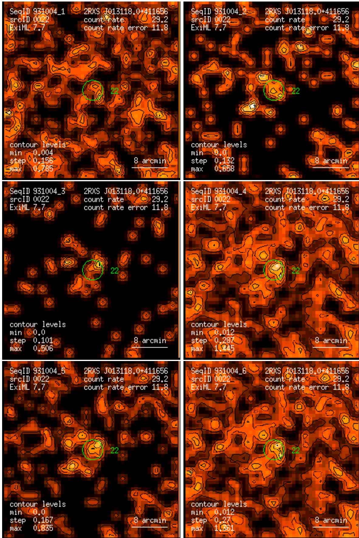
Figure 22: RASS 931004: detection 0022: band rate images, Gaussian filter: (1) PSPC channels 11 – 41, (2) 52 – 90, (3) 91 – 201, (4) 11 – 235, (5) 52 – 201, (6) 11 – 201. Broad band rates in counts/ks. Band rate contour levels in counts/ks/arcmin 2 .
