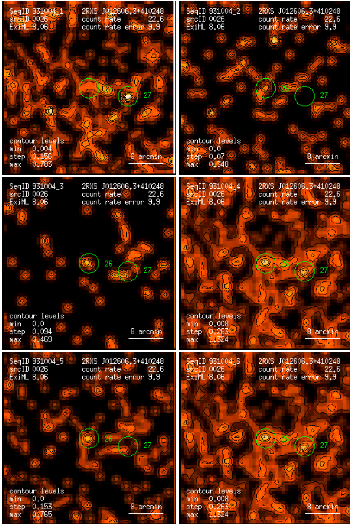
Figure 26: RASS 931004: detection 0026: band rate images, Gaussian filter: (1) PSPC channels 11 – 41, (2) 52 – 90, (3) 91 – 201, (4) 11 – 235, (5) 52 – 201, (6) 11 – 201. Broad band rates in counts/ks. Band rate contour levels in counts/ks/arcmin 2 .
