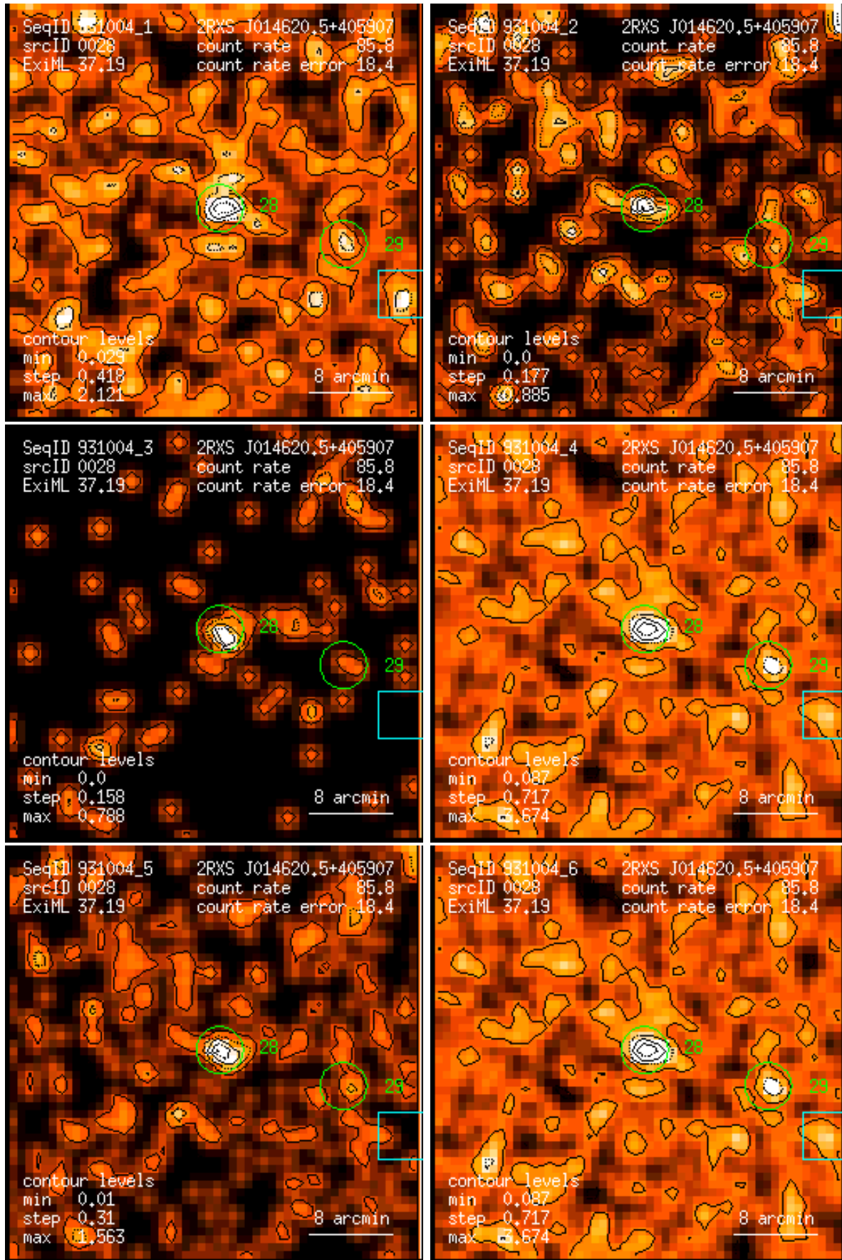
Figure 28: RASS 931004: detection 0028: band rate images, Gaussian filter: (1) PSPC channels 11 – 41, (2) 52 – 90, (3) 91 – 201, (4) 11 – 235, (5) 52 – 201, (6) 11 – 201. Broad band rates in counts/ks. Band rate contour levels in counts/ks/arcmin 2 .
