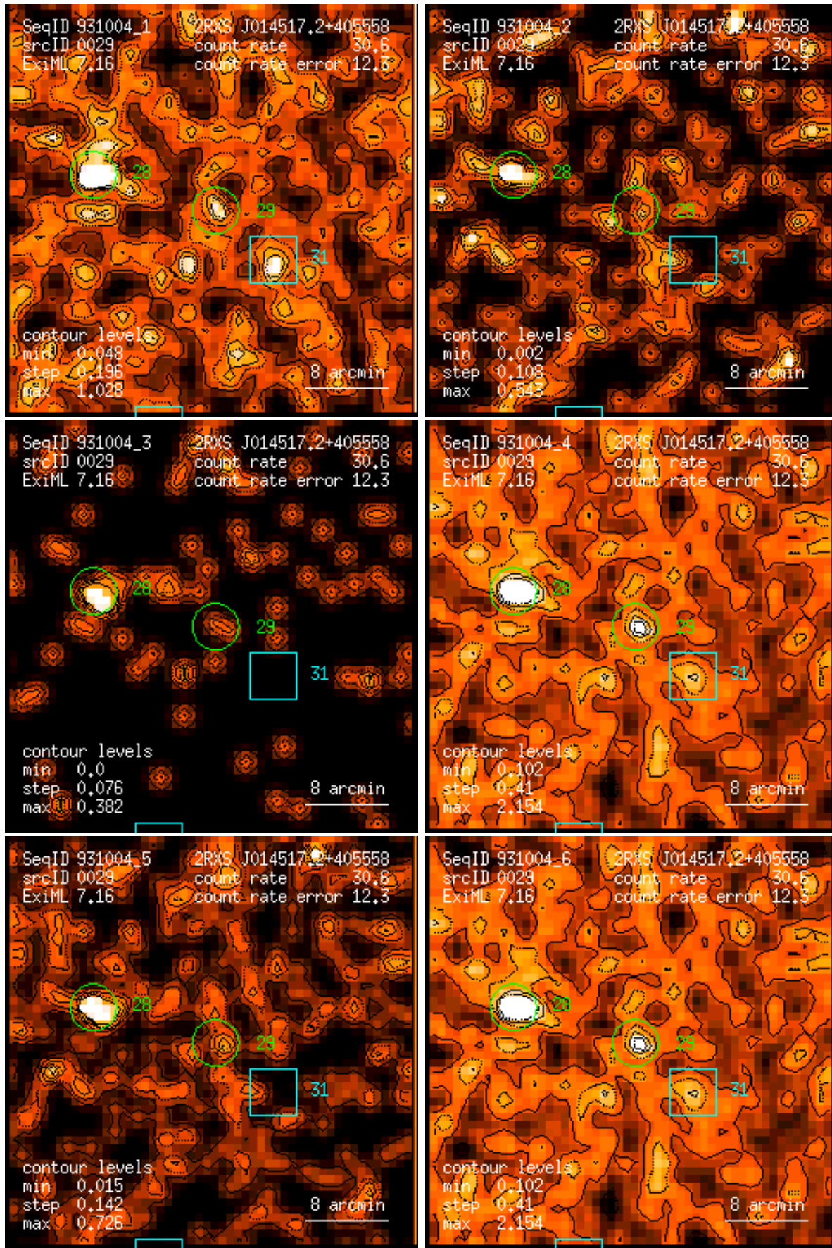
Figure 29: RASS 931004: detection 0029: band rate images, Gaussian filter: (1) PSPC channels 11 – 41, (2) 52 – 90, (3) 91 – 201, (4) 11 – 235, (5) 52 – 201, (6) 11 – 201. Broad band rates in counts/ks. Band rate contour levels in counts/ks/arcmin 2 .
