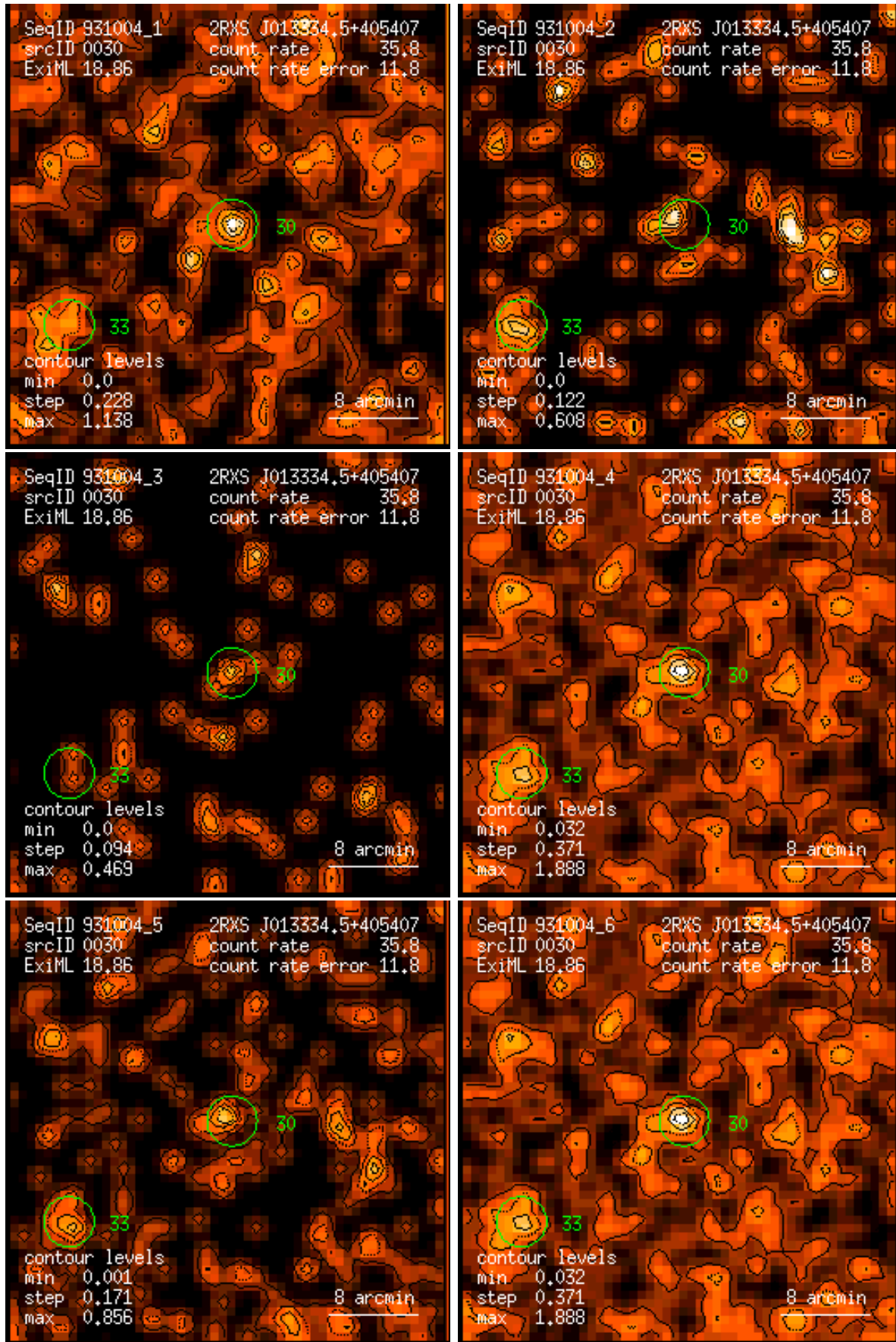
Figure 30: RASS 931004: detection 0030: band rate images, Gaussian filter: (1) PSPC channels 11 – 41, (2) 52 – 90, (3) 91 – 201, (4) 11 – 235, (5) 52 – 201, (6) 11 – 201. Broad band rates in counts/ks. Band rate contour levels in counts/ks/arcmin 2 .
