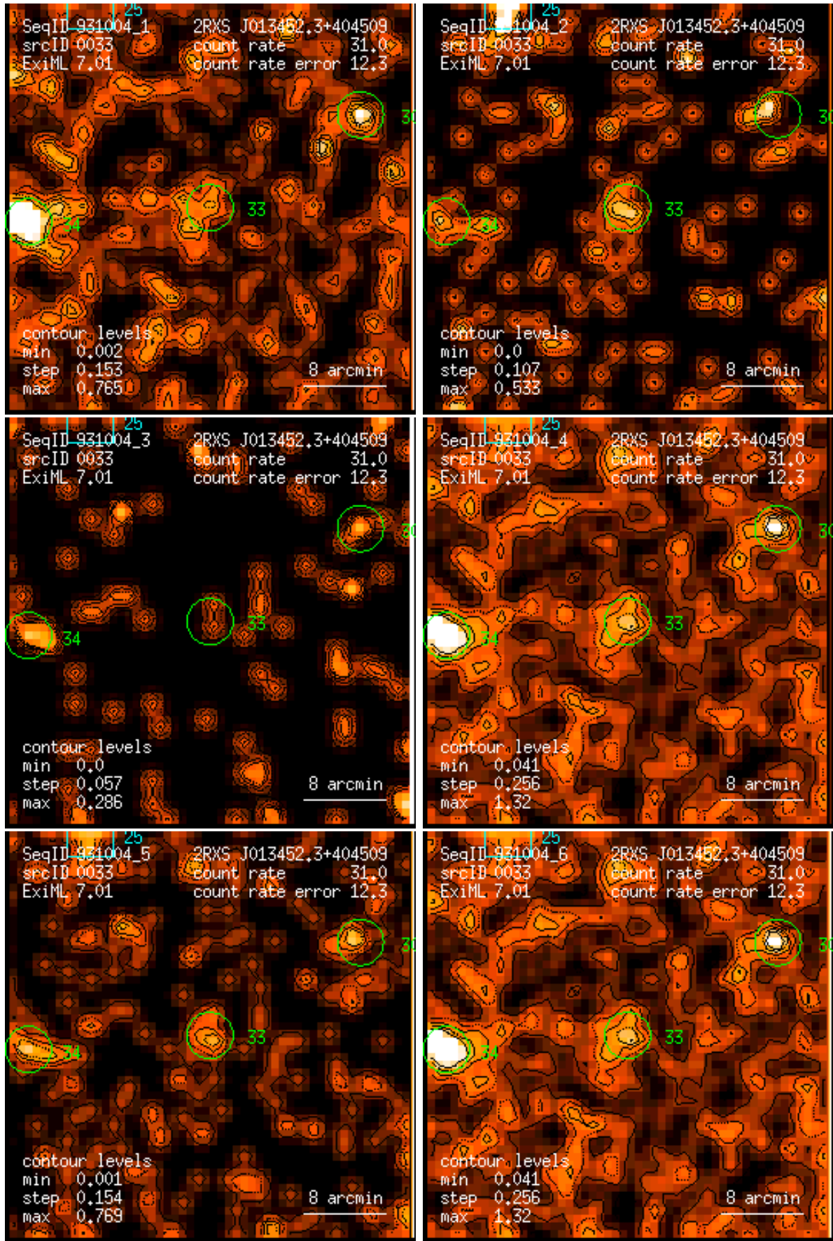
Figure 33: RASS 931004: detection 0033: band rate images, Gaussian filter: (1) PSPC channels 11 – 41, (2) 52 – 90, (3) 91 – 201, (4) 11 – 235, (5) 52 – 201, (6) 11 – 201. Broad band rates in counts/ks. Band rate contour levels in counts/ks/arcmin 2 .
