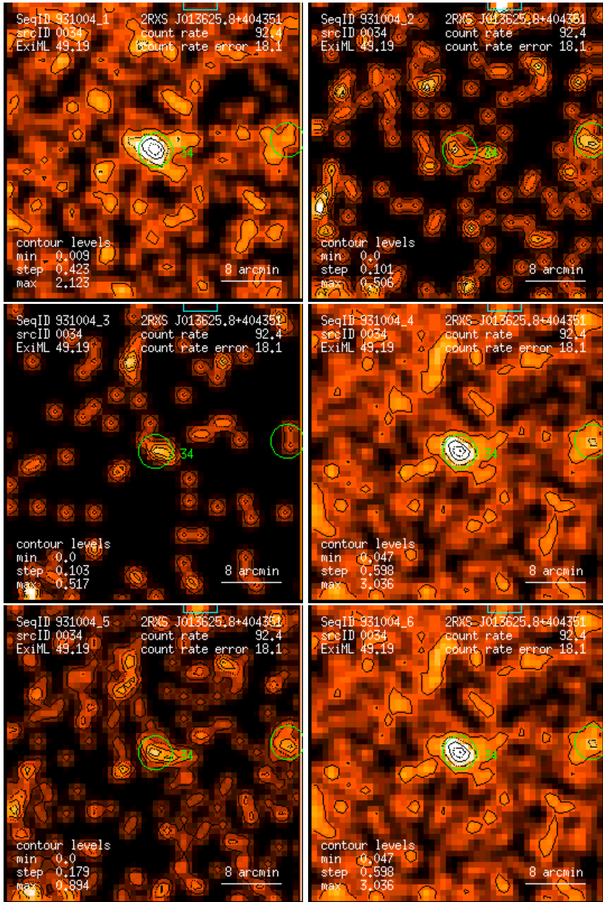
Figure 34: RASS 931004: detection 0034: band rate images, Gaussian filter: (1) PSPC channels 11 – 41, (2) 52 – 90, (3) 91 – 201, (4) 11 – 235, (5) 52 – 201, (6) 11 – 201. Broad band rates in counts/ks. Band rate contour levels in counts/ks/arcmin 2 .
