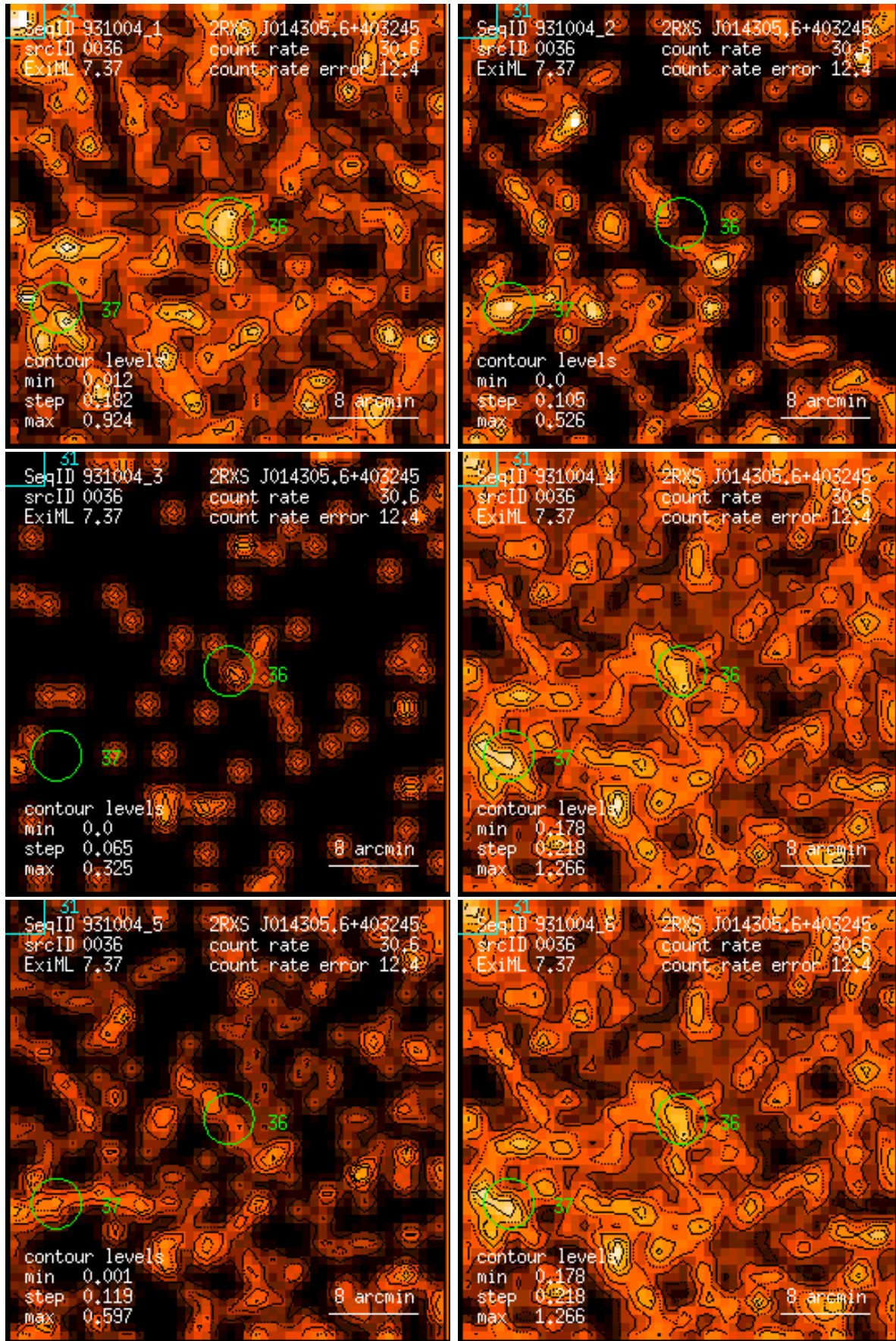
Figure 36: RASS 931004: detection 0036: band rate images, Gaussian filter: (1) PSPC channels 11 – 41, (2) 52 – 90, (3) 91 – 201, (4) 11 – 235, (5) 52 – 201, (6) 11 – 201. Broad band rates in counts/ks. Band rate contour levels in counts/ks/arcmin 2 .
