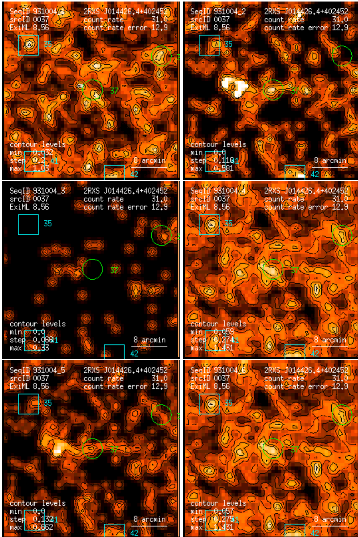
Figure 37: RASS 931004: detection 0037: band rate images, Gaussian filter: (1) PSPC channels 11 – 41, (2) 52 – 90, (3) 91 – 201, (4) 11 – 235, (5) 52 – 201, (6) 11 – 201. Broad band rates in counts/ks. Band rate contour levels in counts/ks/arcmin 2 .
