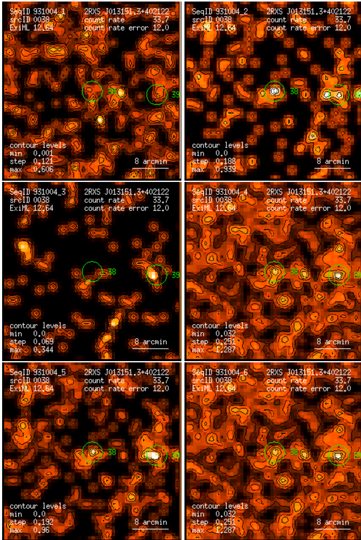
Figure 38: RASS 931004: detection 0038: band rate images, Gaussian filter: (1) PSPC channels 11 – 41, (2) 52 – 90, (3) 91 – 201, (4) 11 – 235, (5) 52 – 201, (6) 11 – 201. Broad band rates in counts/ks. Band rate contour levels in counts/ks/arcmin 2 .
