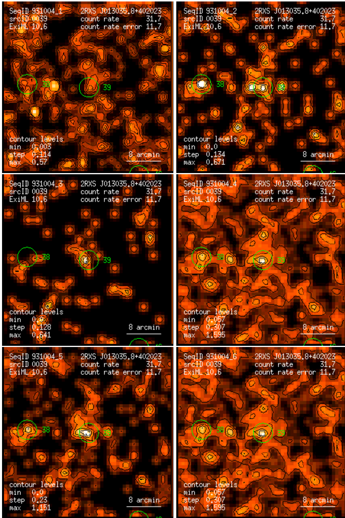
Figure 39: RASS 931004: detection 0039: band rate images, Gaussian filter: (1) PSPC channels 11 – 41, (2) 52 – 90, (3) 91 – 201, (4) 11 – 235, (5) 52 – 201, (6) 11 – 201. Broad band rates in counts/ks. Band rate contour levels in counts/ks/arcmin 2 .
