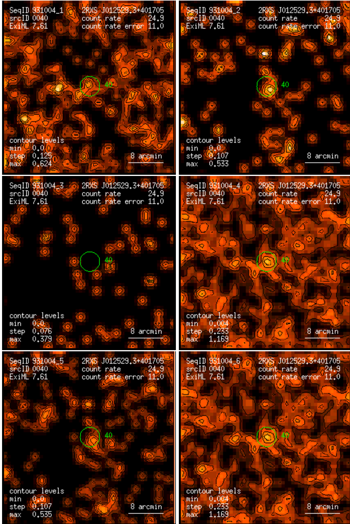
Figure 40: RASS 931004: detection 0040: band rate images, Gaussian filter: (1) PSPC channels 11 – 41, (2) 52 – 90, (3) 91 – 201, (4) 11 – 235, (5) 52 – 201, (6) 11 – 201. Broad band rates in counts/ks. Band rate contour levels in counts/ks/arcmin 2 .
