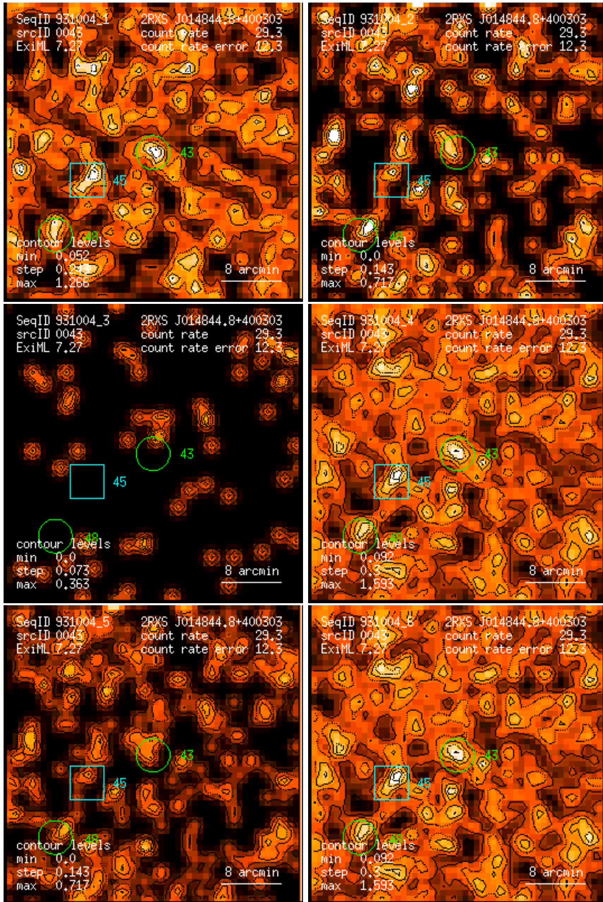
Figure 43: RASS 931004: detection 0043: band rate images, Gaussian filter: (1) PSPC channels 11 – 41, (2) 52 – 90, (3) 91 – 201, (4) 11 – 235, (5) 52 – 201, (6) 11 – 201. Broad band rates in counts/ks. Band rate contour levels in counts/ks/arcmin 2 .
