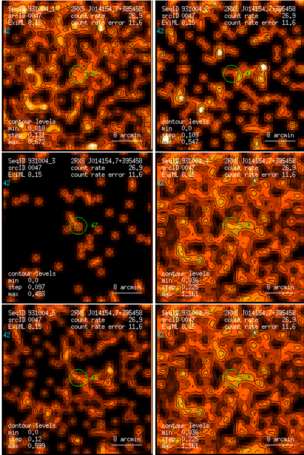
Figure 47: RASS 931004: detection 0047: band rate images, Gaussian filter: (1) PSPC channels 11 – 41, (2) 52 – 90, (3) 91 – 201, (4) 11 – 235, (5) 52 – 201, (6) 11 – 201. Broad band rates in counts/ks. Band rate contour levels in counts/ks/arcmin 2 .
