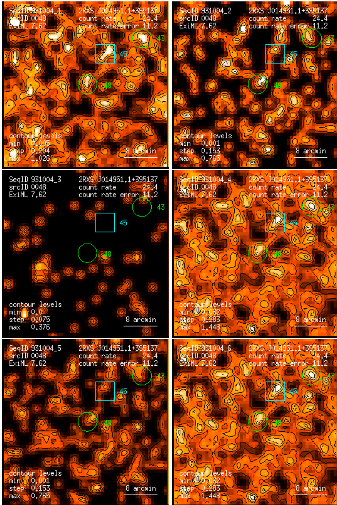
Figure 48: RASS 931004: detection 0048: band rate images, Gaussian filter: (1) PSPC channels 11 – 41, (2) 52 – 90, (3) 91 – 201, (4) 11 – 235, (5) 52 – 201, (6) 11 – 201. Broad band rates in counts/ks. Band rate contour levels in counts/ks/arcmin 2 .
