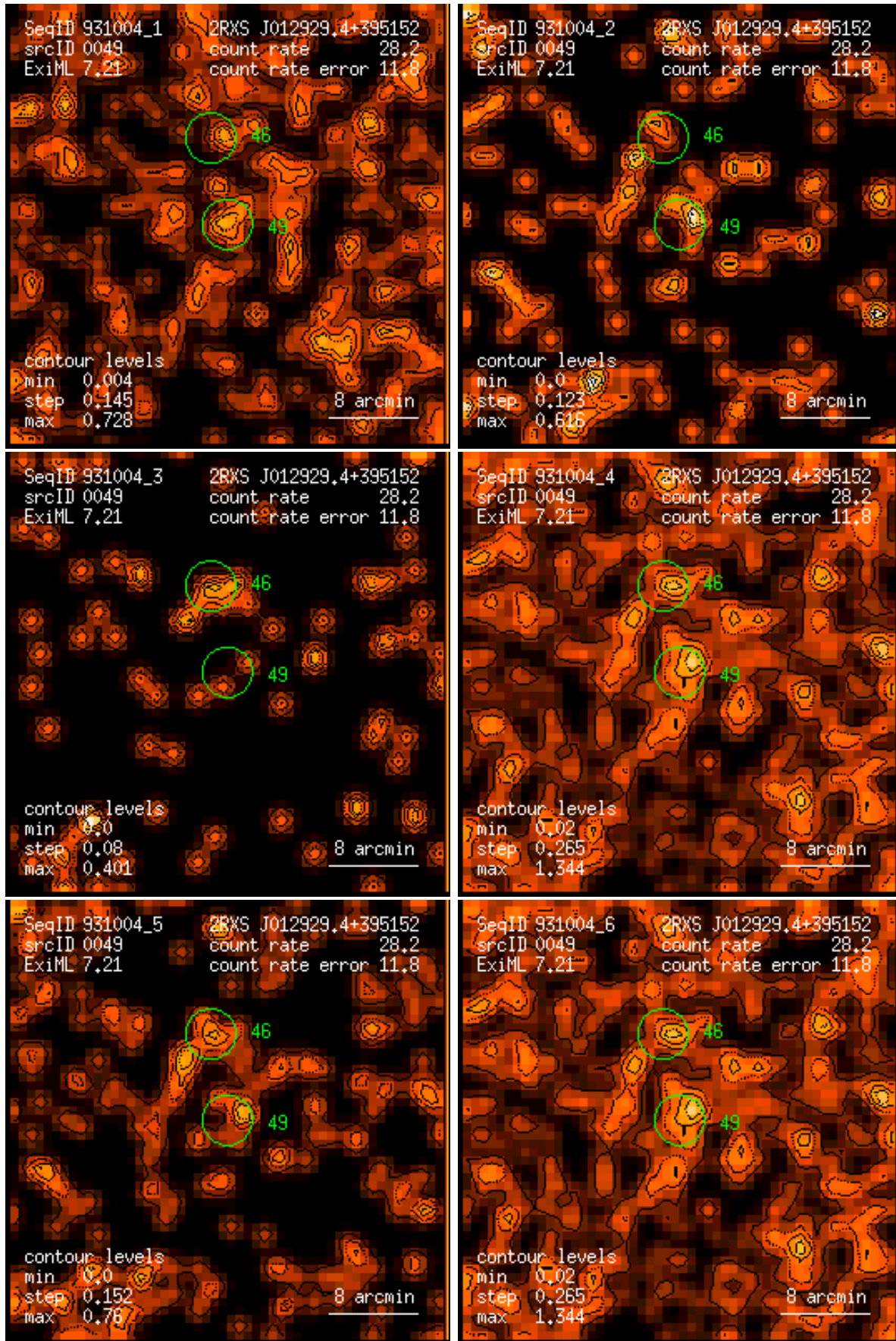
Figure 49: RASS 931004: detection 0049: band rate images, Gaussian filter: (1) PSPC channels 11 – 41, (2) 52 – 90, (3) 91 – 201, (4) 11 – 235, (5) 52 – 201, (6) 11 – 201. Broad band rates in counts/ks. Band rate contour levels in counts/ks/arcmin 2 .
