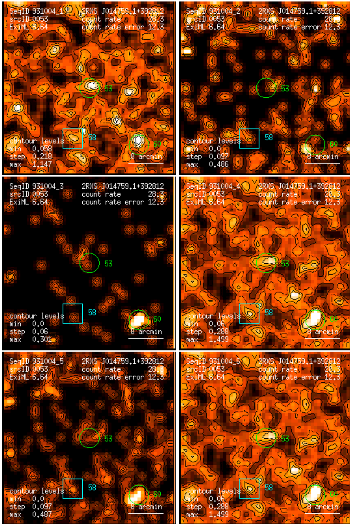
Figure 53: RASS 931004: detection 0053: band rate images, Gaussian filter: (1) PSPC channels 11 – 41, (2) 52 – 90, (3) 91 – 201, (4) 11 – 235, (5) 52 – 201, (6) 11 – 201. Broad band rates in counts/ks. Band rate contour levels in counts/ks/arcmin 2 .
