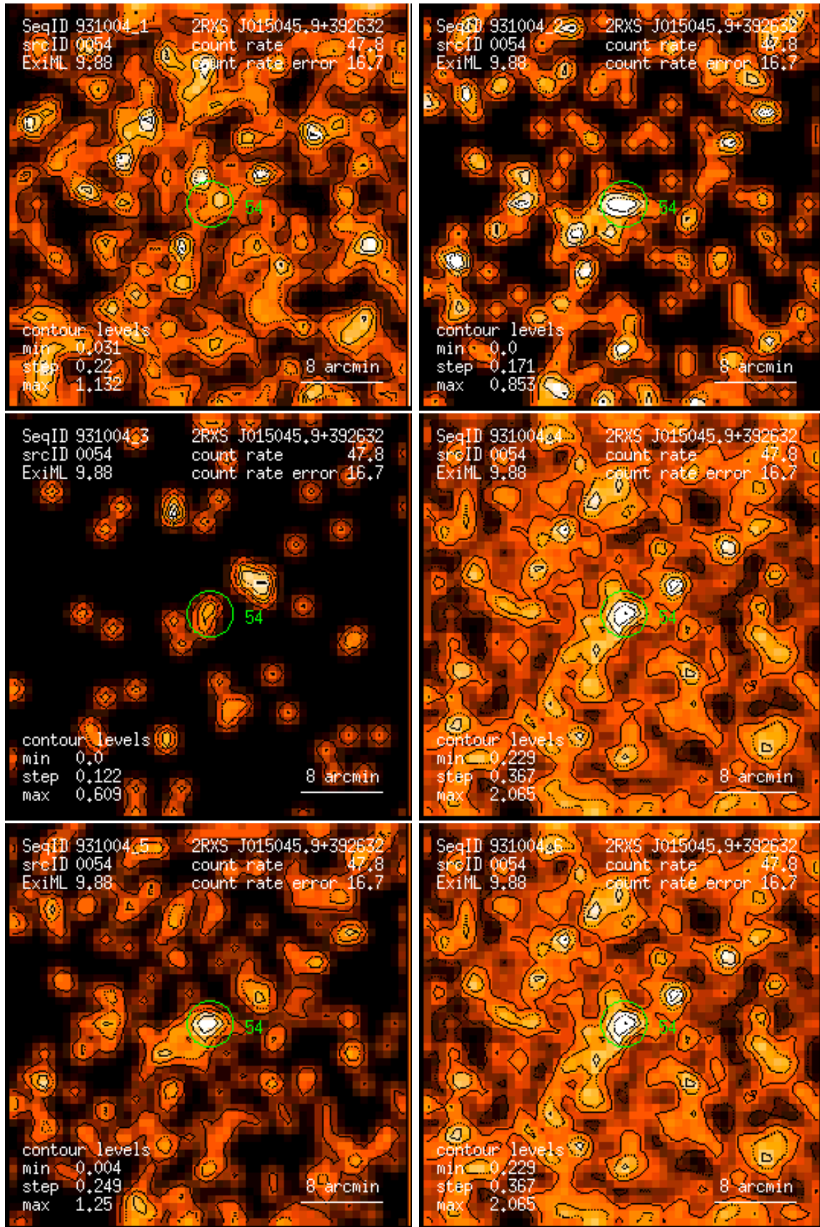
Figure 54: RASS 931004: detection 0054: band rate images, Gaussian filter: (1) PSPC channels 11 – 41, (2) 52 – 90, (3) 91 – 201, (4) 11 – 235, (5) 52 – 201, (6) 11 – 201. Broad band rates in counts/ks. Band rate contour levels in counts/ks/arcmin 2 .
