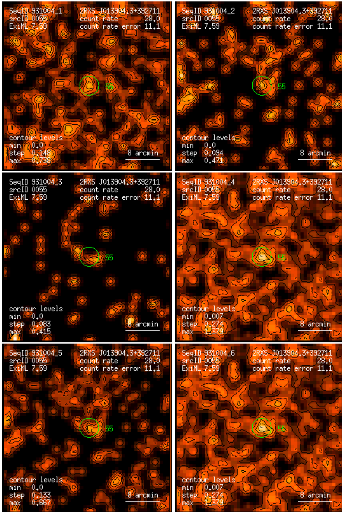
Figure 55: RASS 931004: detection 0055: band rate images, Gaussian filter: (1) PSPC channels 11 – 41, (2) 52 – 90, (3) 91 – 201, (4) 11 – 235, (5) 52 – 201, (6) 11 – 201. Broad band rates in counts/ks. Band rate contour levels in counts/ks/arcmin 2 .
