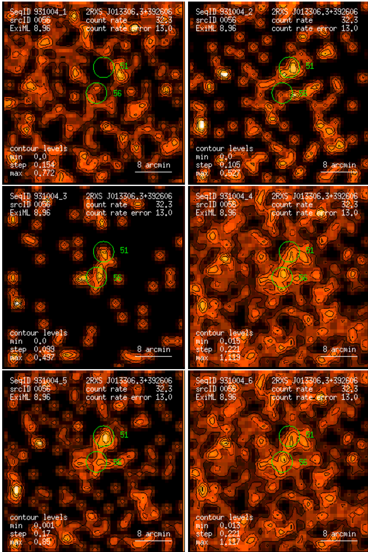
Figure 56: RASS 931004: detection 0056: band rate images, Gaussian filter: (1) PSPC channels 11 – 41, (2) 52 – 90, (3) 91 – 201, (4) 11 – 235, (5) 52 – 201, (6) 11 – 201. Broad band rates in counts/ks. Band rate contour levels in counts/ks/arcmin 2 .
