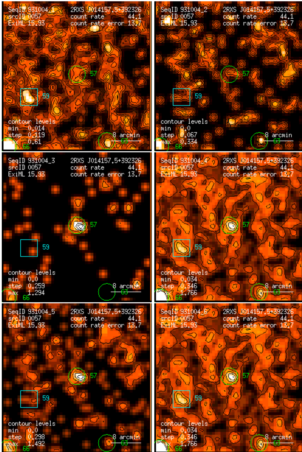
Figure 57: RASS 931004: detection 0057: band rate images, Gaussian filter: (1) PSPC channels 11 – 41, (2) 52 – 90, (3) 91 – 201, (4) 11 – 235, (5) 52 – 201, (6) 11 – 201. Broad band rates in counts/ks. Band rate contour levels in counts/ks/arcmin 2 .
