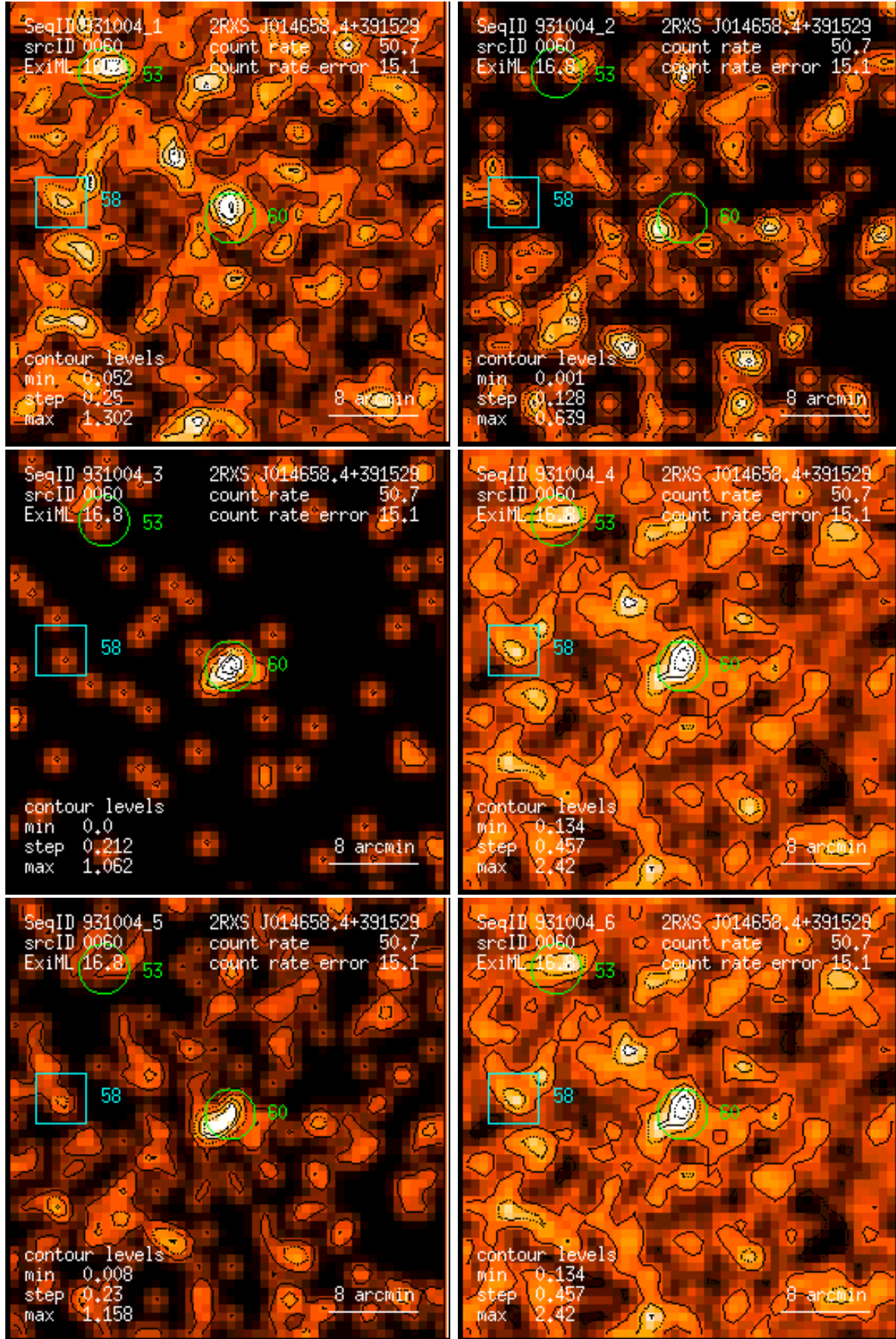
Figure 60: RASS 931004: detection 0060: band rate images, Gaussian filter: (1) PSPC channels 11 – 41, (2) 52 – 90, (3) 91 – 201, (4) 11 – 235, (5) 52 – 201, (6) 11 – 201. Broad band rates in counts/ks. Band rate contour levels in counts/ks/arcmin 2 .
