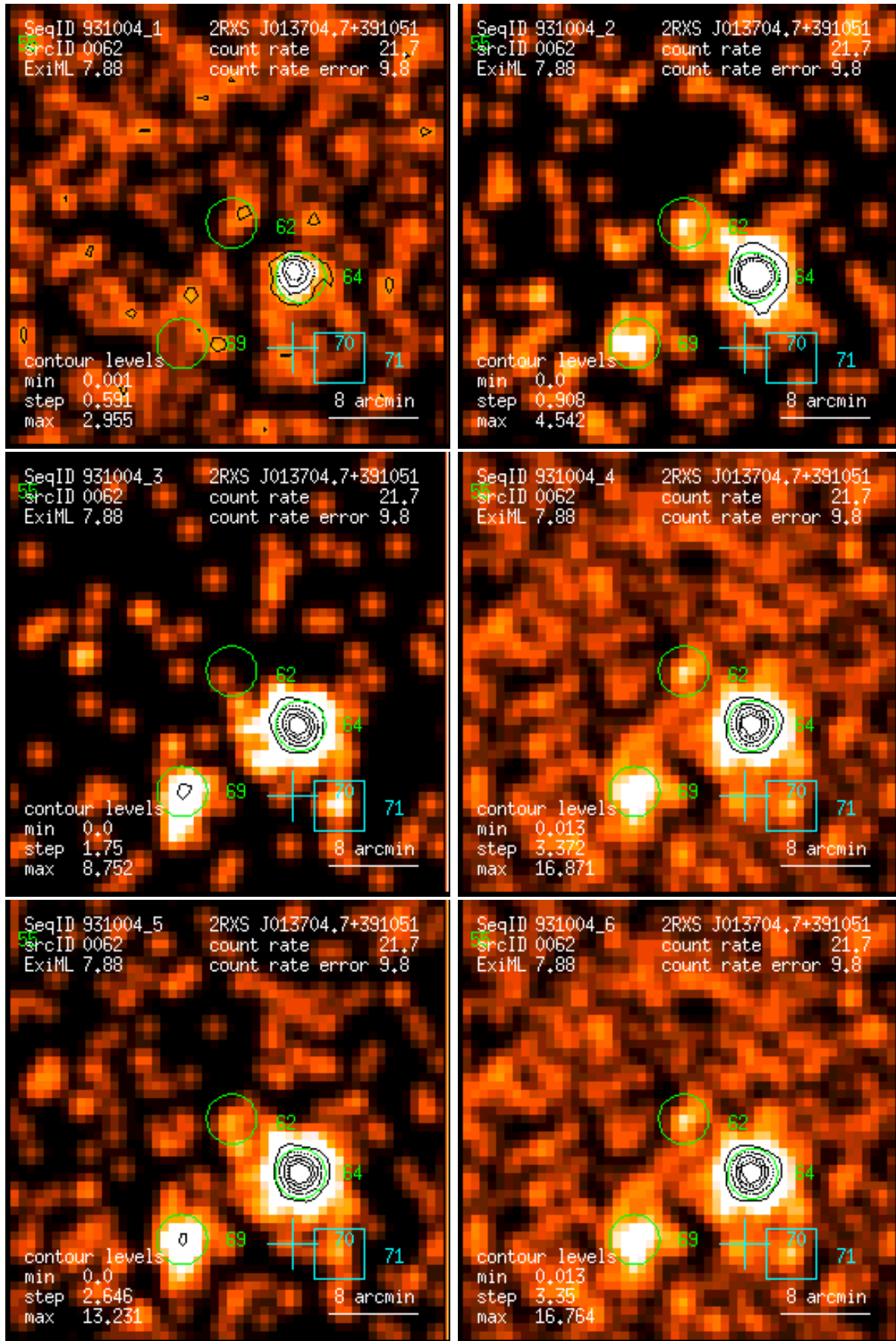
Figure 62: RASS 931004: detection 0062: band rate images, Gaussian filter: (1) PSPC channels 11 – 41, (2) 52 – 90, (3) 91 – 201, (4) 11 – 235, (5) 52 – 201, (6) 11 – 201. Broad band rates in counts/ks. Band rate contour levels in counts/ks/arcmin 2 .
