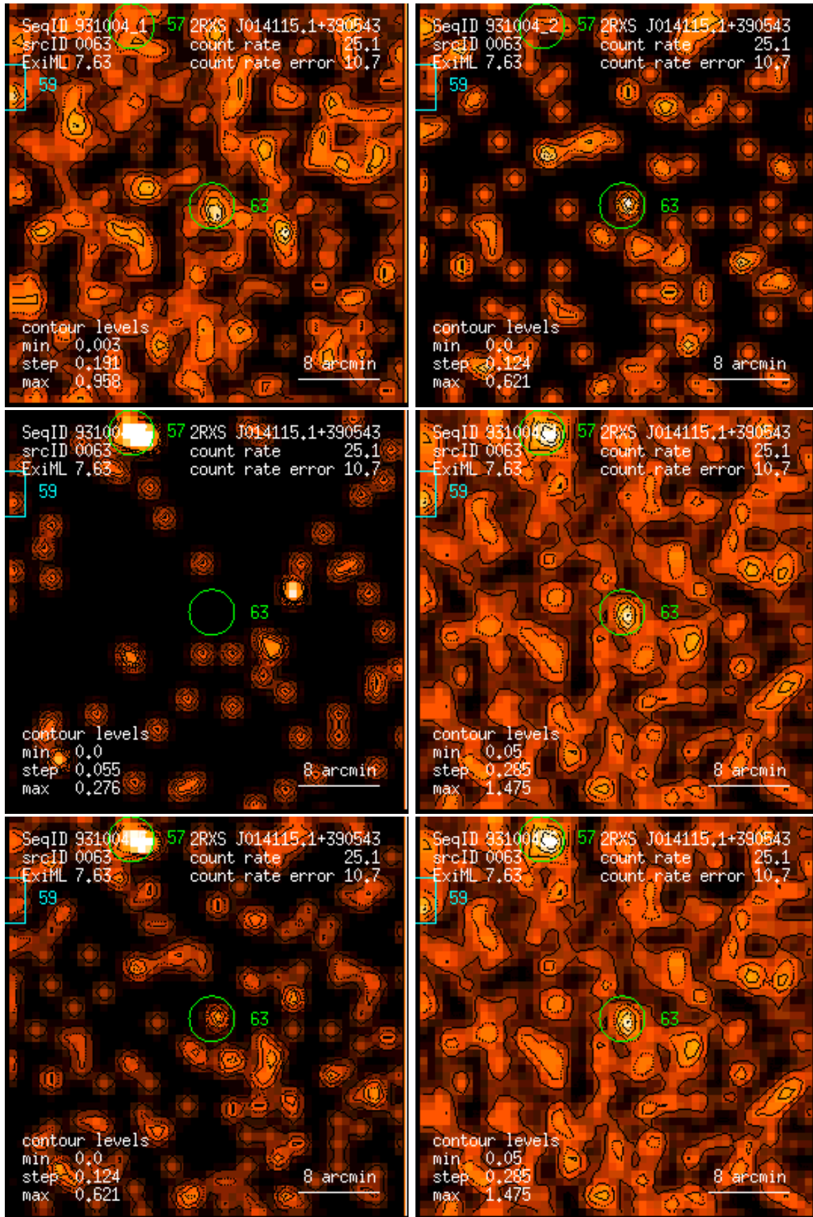
Figure 63: RASS 931004: detection 0063: band rate images, Gaussian filter: (1) PSPC channels 11 – 41, (2) 52 – 90, (3) 91 – 201, (4) 11 – 235, (5) 52 – 201, (6) 11 – 201. Broad band rates in counts/ks. Band rate contour levels in counts/ks/arcmin 2 .
