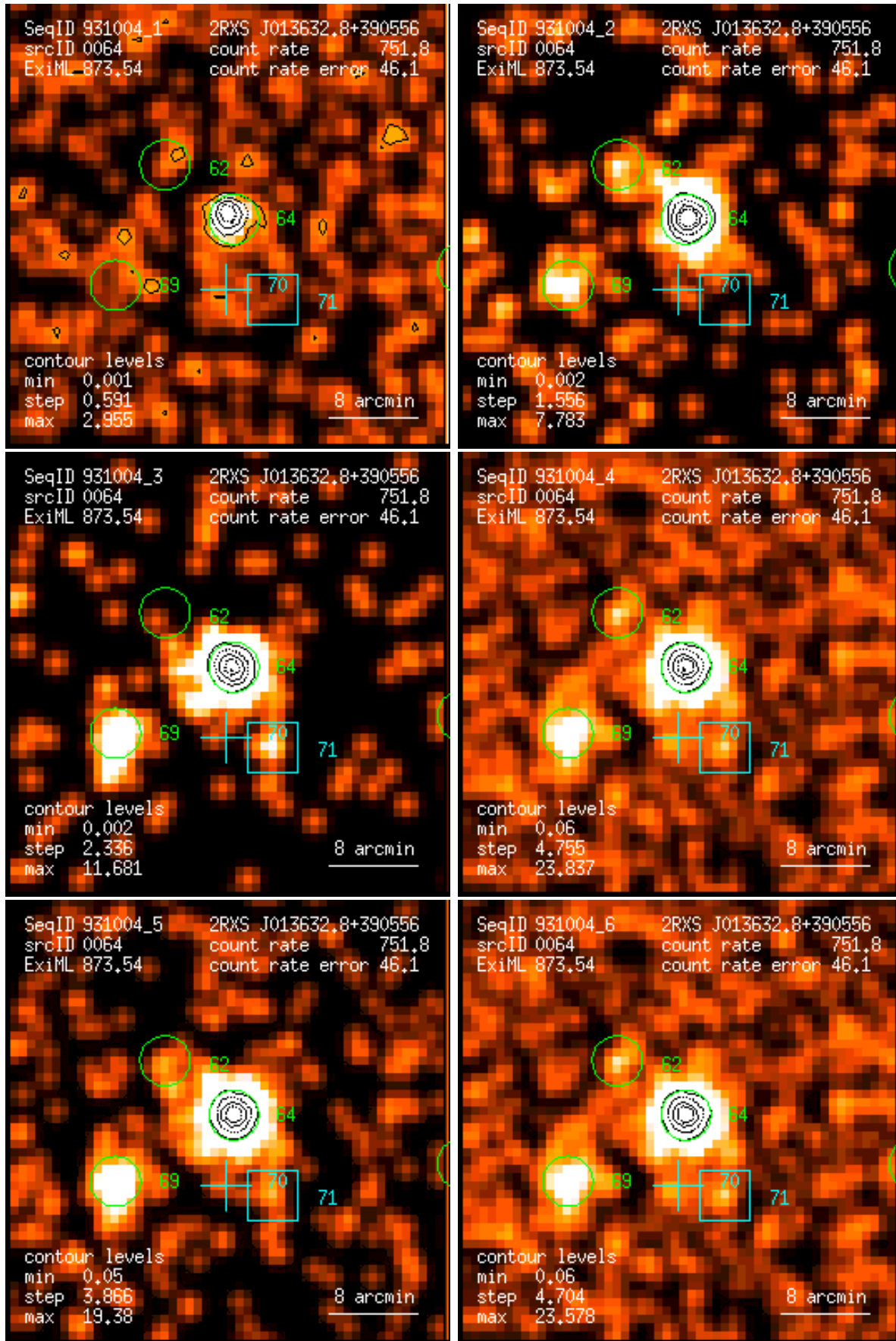
Figure 64: RASS 931004: detection 0064: band rate images, Gaussian filter: (1) PSPC channels 11 – 41, (2) 52 – 90, (3) 91 – 201, (4) 11 – 235, (5) 52 – 201, (6) 11 – 201. Broad band rates in counts/ks. Band rate contour levels in counts/ks/arcmin 2 .
