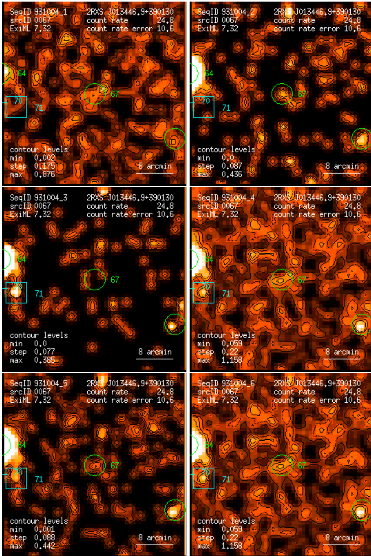
Figure 67: RASS 931004: detection 0067: band rate images, Gaussian filter: (1) PSPC channels 11 – 41, (2) 52 – 90, (3) 91 – 201, (4) 11 – 235, (5) 52 – 201, (6) 11 – 201. Broad band rates in counts/ks. Band rate contour levels in counts/ks/arcmin 2 .
