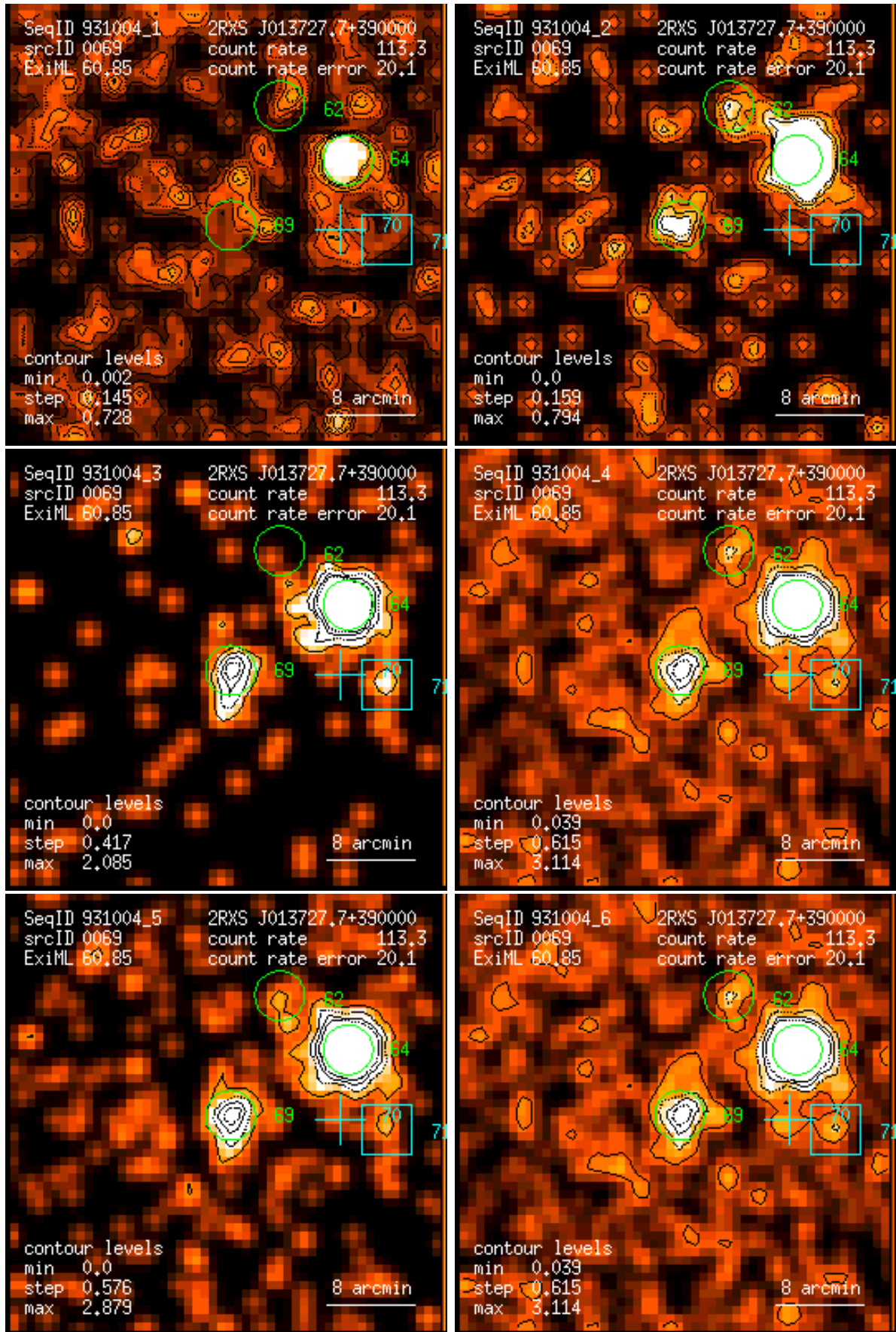
Figure 69: RASS 931004: detection 0069: band rate images, Gaussian filter: (1) PSPC channels 11 – 41, (2) 52 – 90, (3) 91 – 201, (4) 11 – 235, (5) 52 – 201, (6) 11 – 201. Broad band rates in counts/ks. Band rate contour levels in counts/ks/arcmin 2 .
