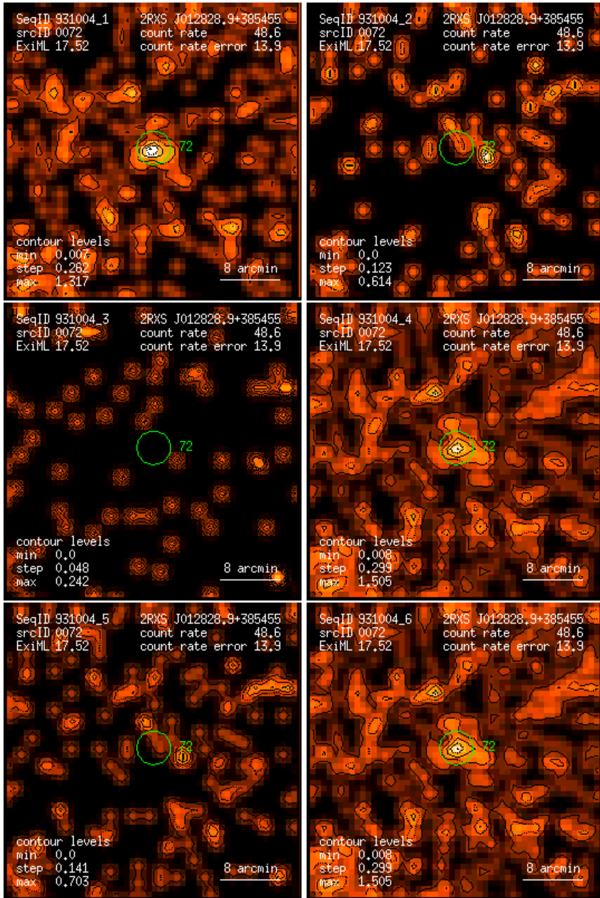
Figure 72: RASS 931004: detection 0072: band rate images, Gaussian filter: (1) PSPC channels 11 – 41, (2) 52 – 90, (3) 91 – 201, (4) 11 – 235, (5) 52 – 201, (6) 11 – 201. Broad band rates in counts/ks. Band rate contour levels in counts/ks/arcmin 2 .
