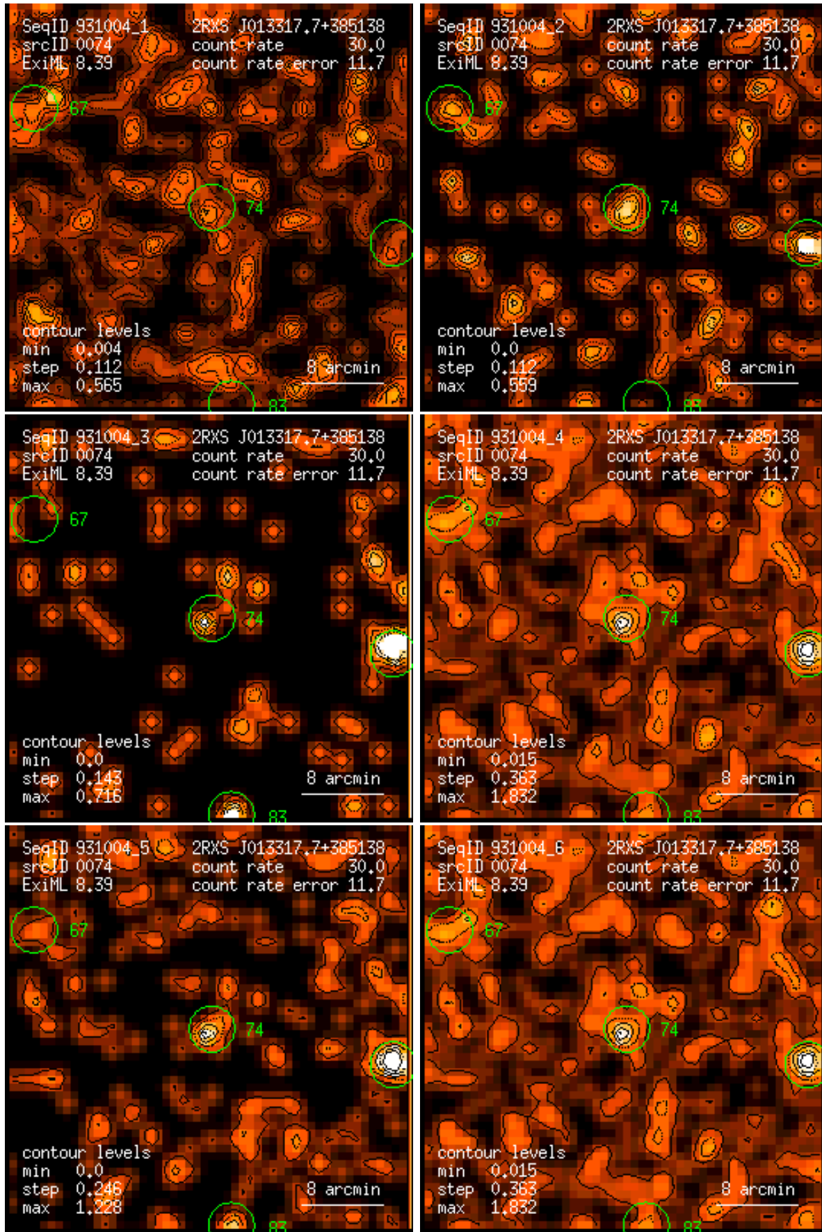
Figure 74: RASS 931004: detection 0074: band rate images, Gaussian filter: (1) PSPC channels 11 – 41, (2) 52 – 90, (3) 91 – 201, (4) 11 – 235, (5) 52 – 201, (6) 11 – 201. Broad band rates in counts/ks. Band rate contour levels in counts/ks/arcmin 2 .
