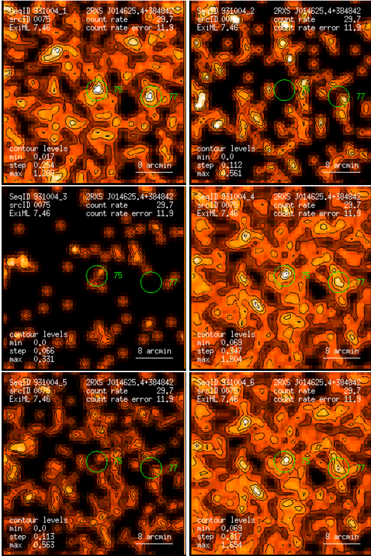
Figure 75: RASS 931004: detection 0075: band rate images, Gaussian filter: (1) PSPC channels 11 – 41, (2) 52 – 90, (3) 91 – 201, (4) 11 – 235, (5) 52 – 201, (6) 11 – 201. Broad band rates in counts/ks. Band rate contour levels in counts/ks/arcmin 2 .
