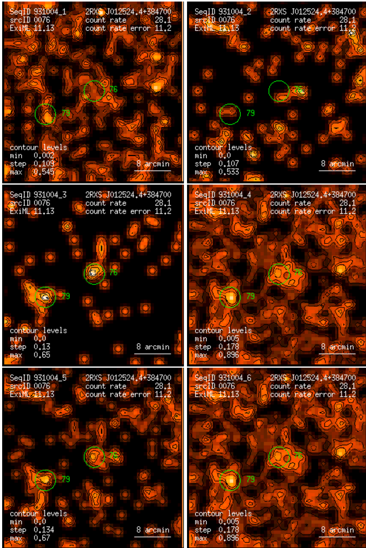
Figure 76: RASS 931004: detection 0076: band rate images, Gaussian filter: (1) PSPC channels 11 – 41, (2) 52 – 90, (3) 91 – 201, (4) 11 – 235, (5) 52 – 201, (6) 11 – 201. Broad band rates in counts/ks. Band rate contour levels in counts/ks/arcmin 2 .
