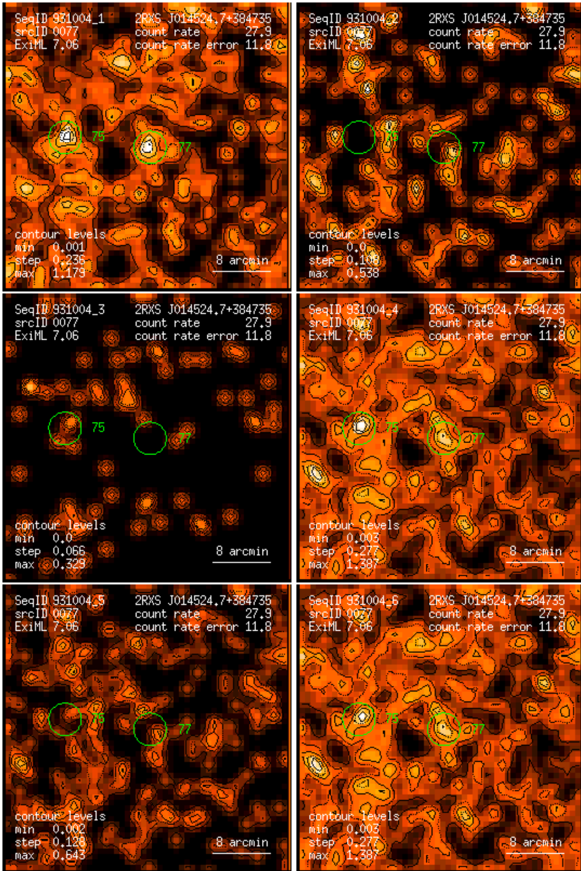
Figure 77: RASS 931004: detection 0077: band rate images, Gaussian filter: (1) PSPC channels 11 – 41, (2) 52 – 90, (3) 91 – 201, (4) 11 – 235, (5) 52 – 201, (6) 11 – 201. Broad band rates in counts/ks. Band rate contour levels in counts/ks/arcmin 2 .
