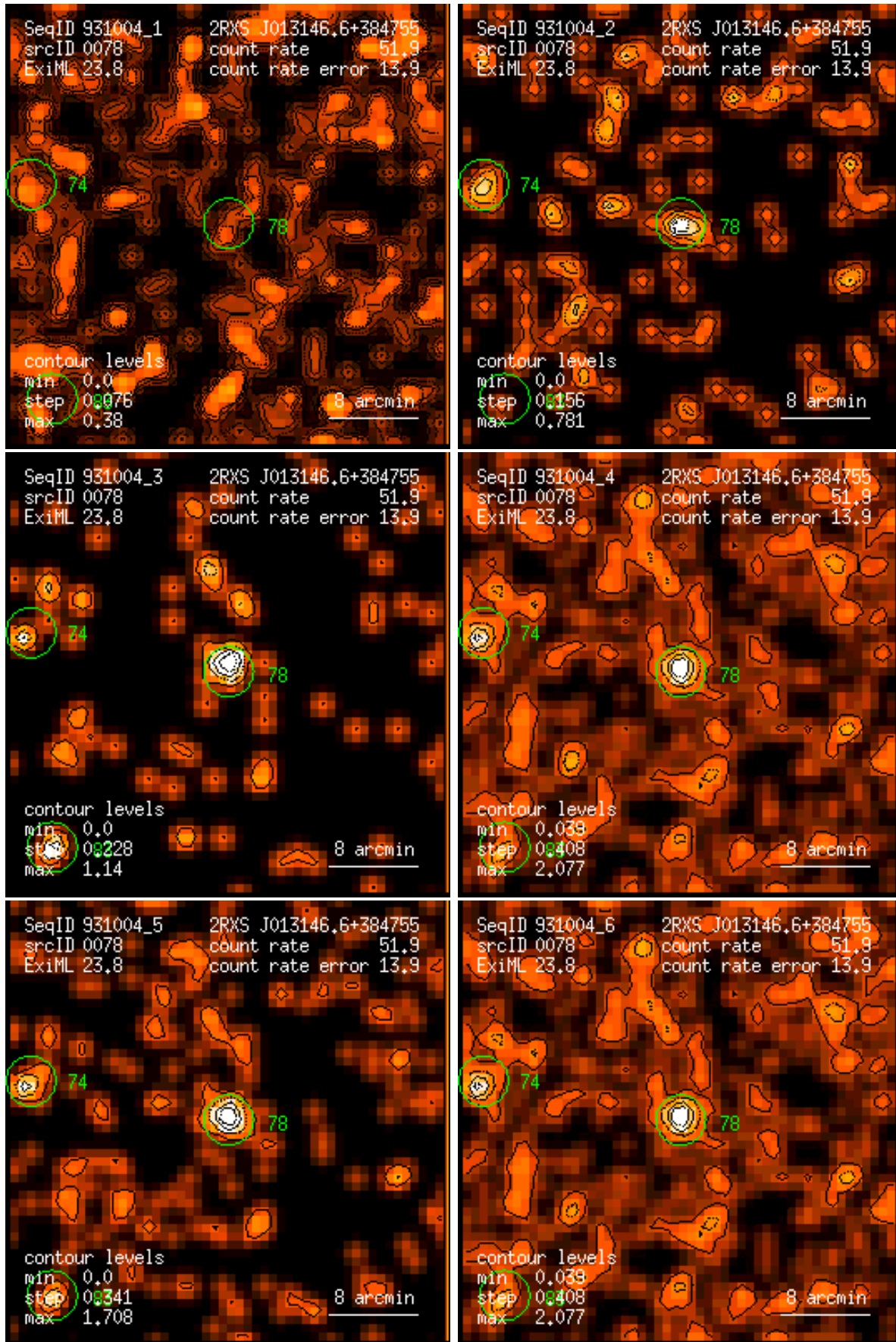
Figure 78: RASS 931004: detection 0078: band rate images, Gaussian filter: (1) PSPC channels 11 – 41, (2) 52 – 90, (3) 91 – 201, (4) 11 – 235, (5) 52 – 201, (6) 11 – 201. Broad band rates in counts/ks. Band rate contour levels in counts/ks/arcmin 2 .
