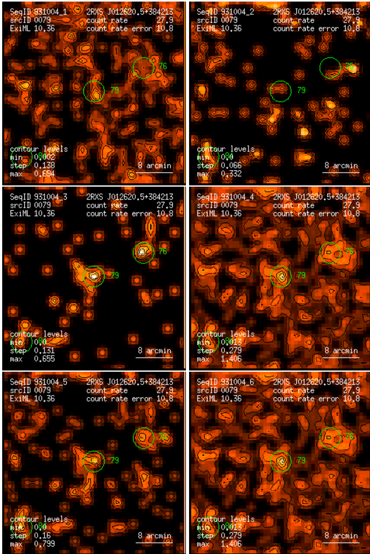
Figure 79: RASS 931004: detection 0079: band rate images, Gaussian filter: (1) PSPC channels 11 – 41, (2) 52 – 90, (3) 91 – 201, (4) 11 – 235, (5) 52 – 201, (6) 11 – 201. Broad band rates in counts/ks. Band rate contour levels in counts/ks/arcmin 2 .
