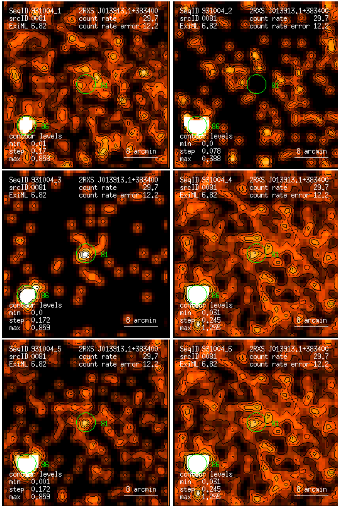
Figure 81: RASS 931004: detection 0081: band rate images, Gaussian filter: (1) PSPC channels 11 – 41, (2) 52 – 90, (3) 91 – 201, (4) 11 – 235, (5) 52 – 201, (6) 11 – 201. Broad band rates in counts/ks. Band rate contour levels in counts/ks/arcmin 2 .
