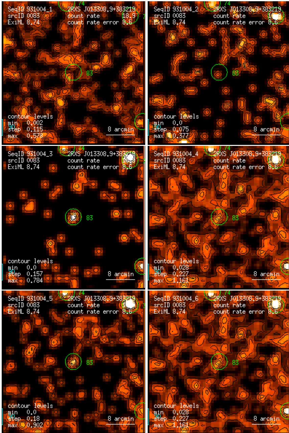
Figure 83: RASS 931004: detection 0083: band rate images, Gaussian filter: (1) PSPC channels 11 – 41, (2) 52 – 90, (3) 91 – 201, (4) 11 – 235, (5) 52 – 201, (6) 11 – 201. Broad band rates in counts/ks. Band rate contour levels in counts/ks/arcmin 2 .
