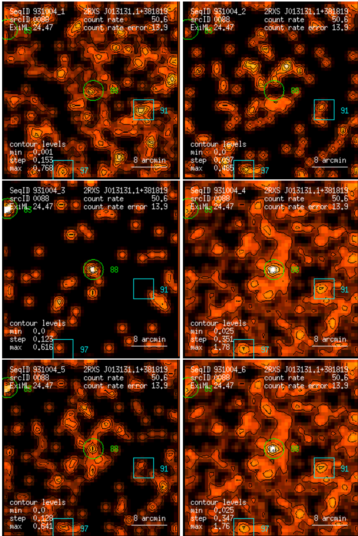
Figure 88: RASS 931004: detection 0088: band rate images, Gaussian filter: (1) PSPC channels 11 – 41, (2) 52 – 90, (3) 91 – 201, (4) 11 – 235, (5) 52 – 201, (6) 11 – 201. Broad band rates in counts/ks. Band rate contour levels in counts/ks/arcmin 2 .
