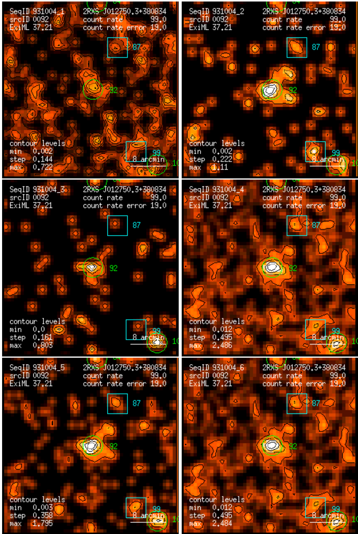
Figure 92: RASS 931004: detection 0092: band rate images, Gaussian filter: (1) PSPC channels 11 – 41, (2) 52 – 90, (3) 91 – 201, (4) 11 – 235, (5) 52 – 201, (6) 11 – 201. Broad band rates in counts/ks. Band rate contour levels in counts/ks/arcmin 2 .
