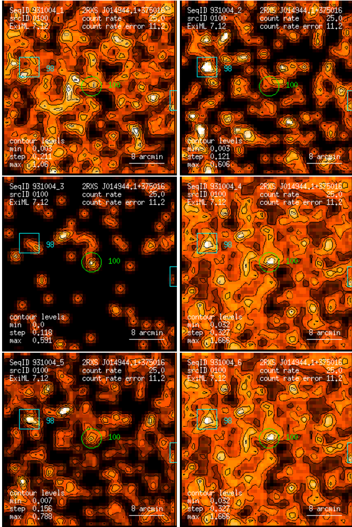
Figure 100: RASS 931004: detection 0100: band rate images, Gaussian filter: (1) PSPC channels 11 – 41, (2) 52 – 90, (3) 91 – 201, (4) 11 – 235, (5) 52 – 201, (6) 11 – 201. Broad band rates in counts/ks. Band rate contour levels in counts/ks/arcmin 2 .
