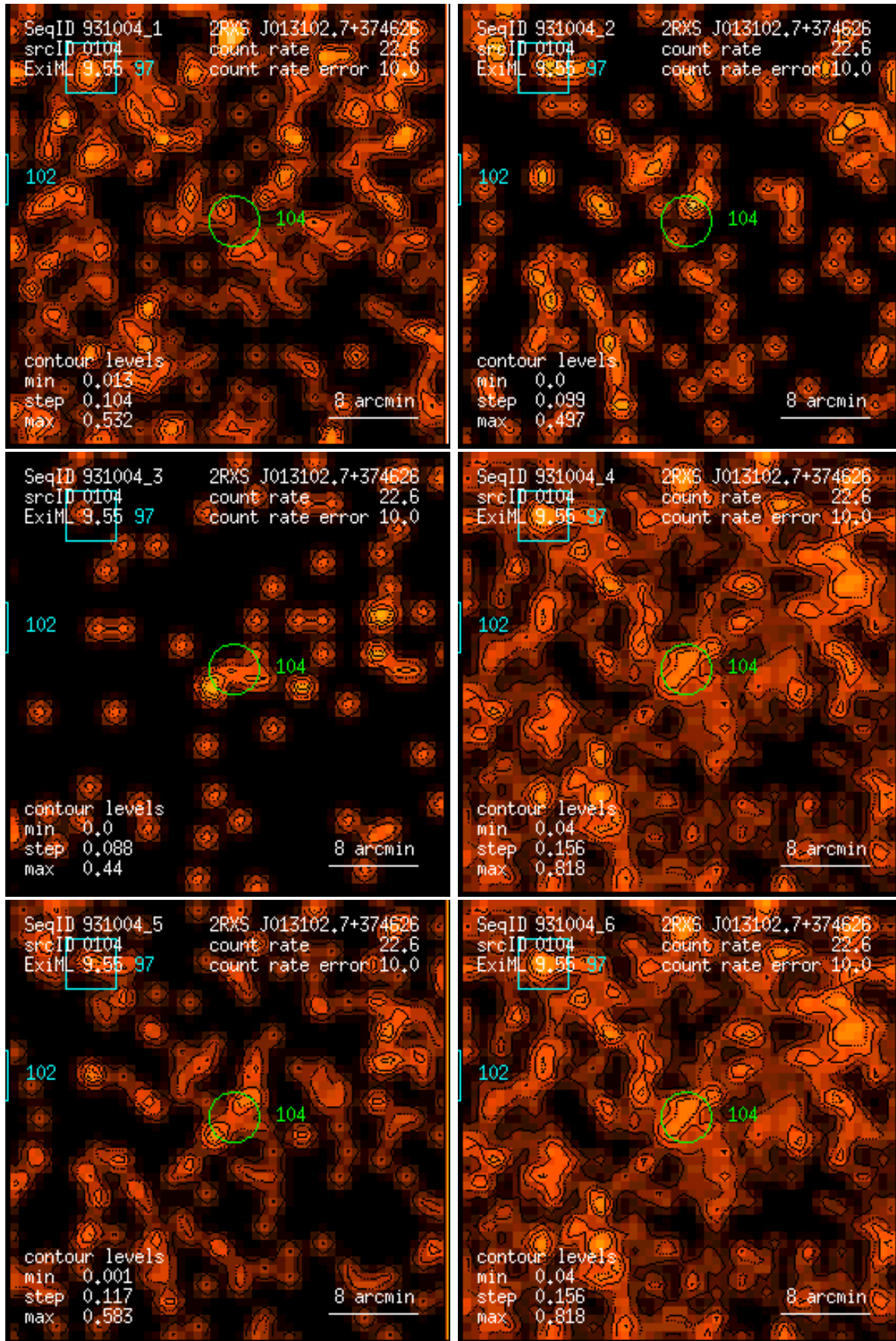
Figure 104: RASS 931004: detection 0104: band rate images, Gaussian filter: (1) PSPC channels 11 – 41, (2) 52 – 90, (3) 91 – 201, (4) 11 – 235, (5) 52 – 201, (6) 11 – 201. Broad band rates in counts/ks. Band rate contour levels in counts/ks/arcmin 2 .
