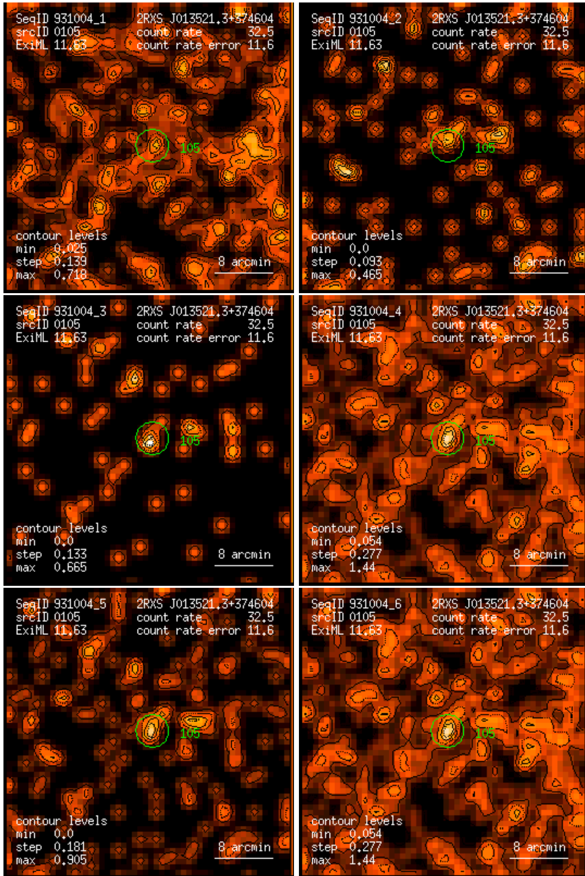
Figure 105: RASS 931004: detection 0105: band rate images, Gaussian filter: (1) PSPC channels 11 – 41, (2) 52 – 90, (3) 91 – 201, (4) 11 – 235, (5) 52 – 201, (6) 11 – 201. Broad band rates in counts/ks. Band rate contour levels in counts/ks/arcmin 2 .
